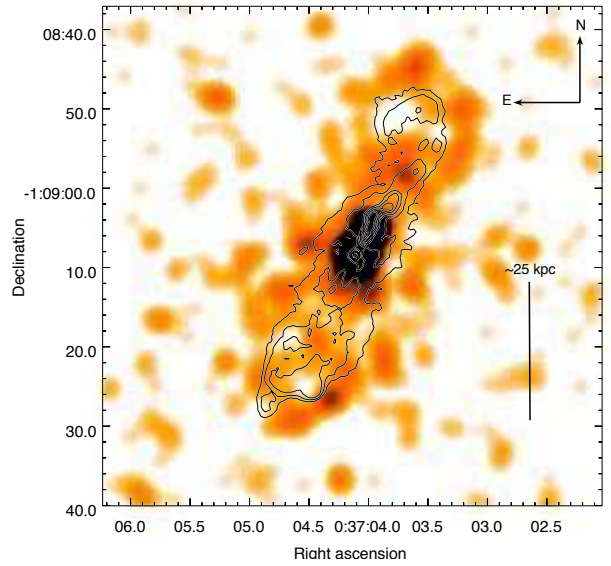
Figure 1. PKS 0034–01 (3C 15). The radio contours increase by factors of 2 between 0.0001 and 0.0128 Jy/beam, the beam major axis is 0.3 arcsec, and the minor axis is 0.3 arcsec.
