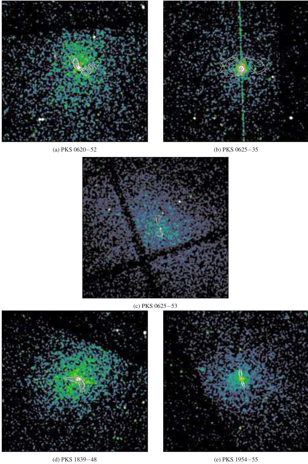
Figure 29. Zoomed-out X-ray images illustrating the dense environments of the FRI LERGs in the low- z 2Jy sample. All the images are smoothed with a Gaussian profile with \sigma = 7 pixels (1 pixel=0.492 arcsec). PKS 0915–11 (Hydra A) and PKS 1648+05 (Hercules A) are not included, as their environments can already be clearly seen in Figs. 13 and 16. We have not included here the FRII LERGs, as the environment of PKS 2211–17 (3C 444) can be clearly seen in Fig. 24, and PKS 0034–01 (3C 15) and PKS 0043–42, whose nuclear spectra are atypical for LERGs, show no clear signs of extended emission.
