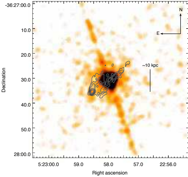
Figure 8. PKS 0521–36. The radio contours increase by factors of 2 between 0.02 and 2.56 Jy/beam, the beam major axis is 1.3 arcsec, and the minor axis is 0.7 arcsec. The instrumental streak is visible in the NE-SW direction.
