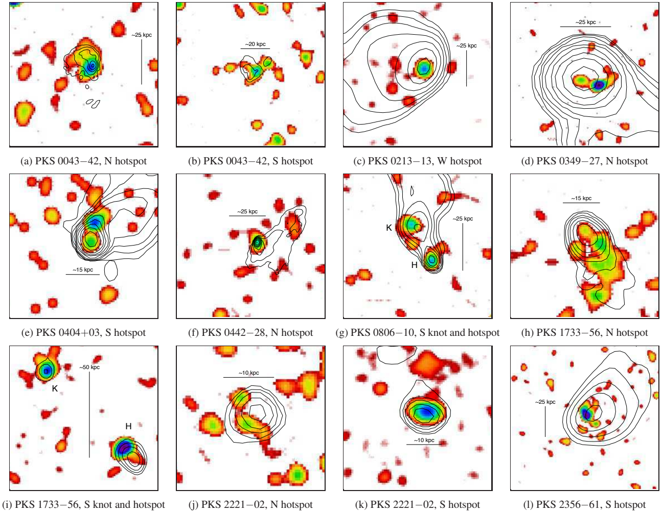
Figure 27. X-ray hotspot close-ups for the sources in Table 2. The radio contours are the same as those detailed in the captions of Figs. 1 to 26. All the images are lightly smoothed with a Gaussian profile with \sigma = 5 pixels (1 pixel=0.492 arcsec). Where both a knot and a hotspot are present in the image, they have been labelled, respectively, as ‘K’ and ‘H’. The hotspots of PKS 0945+07 (3C 227), PKS 1559+02 (3C 327), and PKS 1949+02 (3C 403) are not displayed, as they are discussed in detail in the original publications (Hardcastle et al. 2007b; Kraft et al. 2005).
