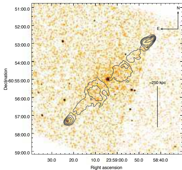
Figure 26. PKS 2356–61. The radio contours increase by factors of 2 between 0.02 and 0.64 Jy/beam, the beam major axis is 7.2 arcsec, and the minor axis is 6.9 arcsec.
