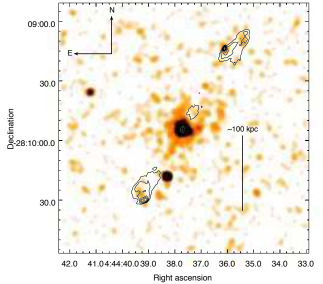
Figure 7. PKS 0442–28. The radio contours increase by factors of 2 between 0.001 and 0.128 Jy/beam, the beam major axis is 1.0 arcsec, and the minor axis is 0.6 arcsec.
