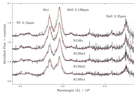
Figure 6. Rectified, spatially resolved near-IR (VLT/SINFONI, Schnurr et al. 2009) spectroscopy of R136 WN5h stars (black) together with synthetic spectra, accounting for instrumental broadening ( 100 \text{ km s}^{-1} ) plus rotational broadening of 200 \text{ km s}^{-1} for R136a2, a3 and c. Consistent hydrogen contents are obtained from the peak intensity ratio of \text{Br}\gamma/\text{HeII } 2.189\mu\text{m} and optical (Pickering-Balmer series) diagnostics. Nitrogen emission includes \text{N V } 2.100\mu\text{m} and \text{N III } 2.103 - 2.115\mu\text{m} .
