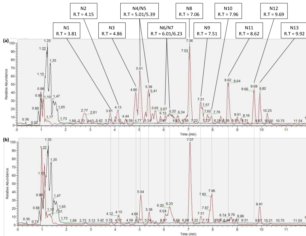
Figure 1: Negative ionisation mode chromatogram of SOA generated from the ozonolysis of \alpha -phellandrene in (a) a standard experiment and (b) an experiment that had formic acid added as a stabilised CI scavenger. Red line represents sample whilst black line is a preconditioned blank filter. Major negative mode ionisation peaks detected across all experiments (Table 2) are labelled.
