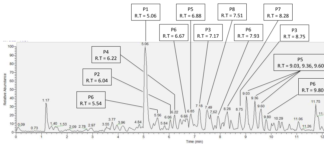
5 Figure 5: Positive ionisation mode chromatogram of SOA generated from the ozonolysis of \alpha -phellandrene. Major positive mode ionisation peaks detected across all experiments (Table 3) are labelled.
