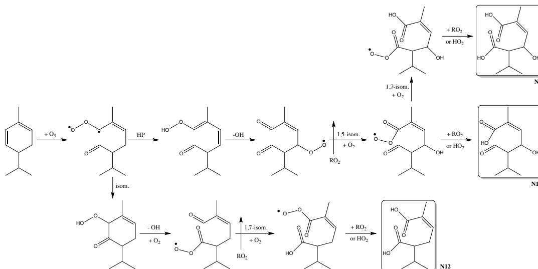
Figure 4: Formation mechanisms of compounds N9 and N12.
