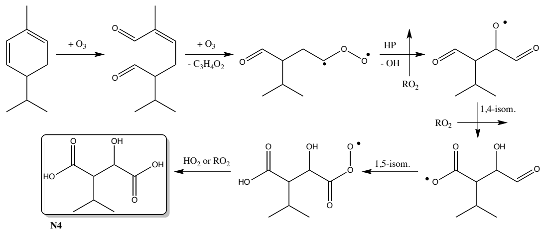
Figure 3: Proposed formation mechanism of compound N4. N5 is formed through an analogous mechanism starting with initial attack of ozone at the more substituted double bond.
