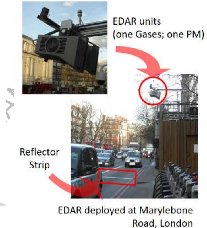
Figure 1: Left, schematic of HEAT EDAR VERSS showing main components. The EDAR systems is activated when a forward-facing camera detects an on-coming vehicle and rapidly whiskbroom scans back and forth along the road mounted reflector strip repeatedly as the vehicle passes over to generate plume images of measured species. Simultaneously, a meteorological monitor records ambient temperature, pressure and humidity, an automatic number plate recognition system and speed camera logs vehicle information. Right, photographs of the EDAR deployment of Marylebone Road London, where the unit was deployed on the roof of an air quality monitoring station.
