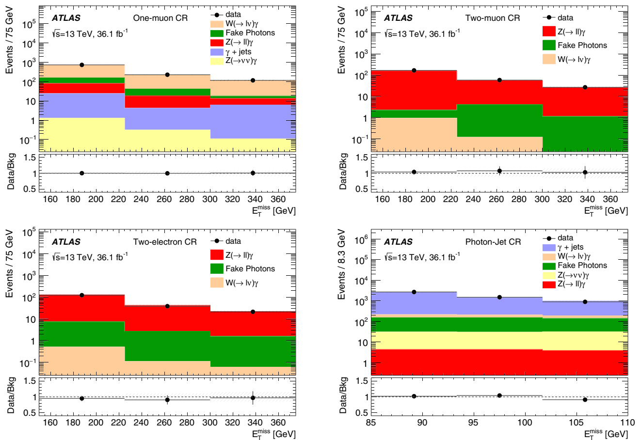
Fig. 2 Distribution of E_T^{\text{miss}} in data and for the expected total background in the CRs: 1muCR (top left), 2muCR (top right), 2eleCR (bottom left) and PhJetCR (bottom right). In 1muCR and 2muCR, the muons are treated as non-interacting particles in the E_T^{\text{miss}} reconstruction; the electrons are handled similarly in 2eleCR. The total background expectation is normalised using the scale factors k' derived from the multiple-
