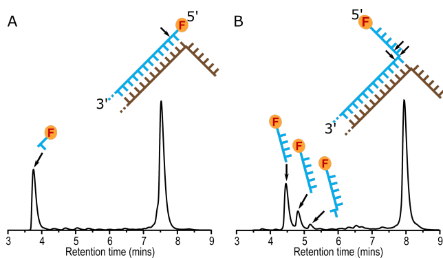
Figure 2. Products of hEXO1-352-catalyzed reactions as determined by HPLC. Chromatograms of hEXO1-352 reaction on (A) 3'-overhang and (B) psY substrates bearing 5' fluorescein labels produces (A) a single nucleotide product and (B) three ss products corresponding to reaction one nucleotide into the duplex, the ss-ds junction and one nucleotide into the flap (6, 5 & 4 nucleotides, respectively). Schematic representations of fluorescein-labelled products and substrates are shown.
