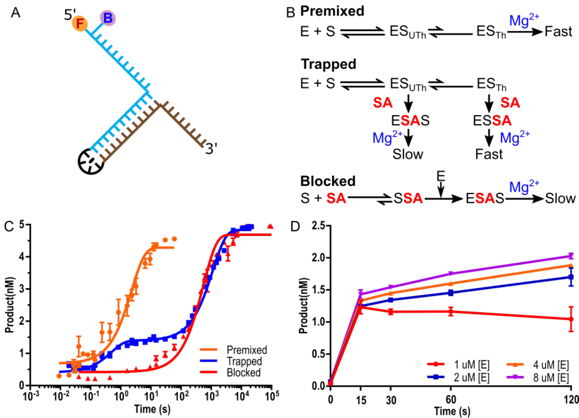
Figure 3. Streptavidin trapping and blocking experiments of EXO1 substrates reveals role for threading in the hEXO1-352-catalyzed endonucleolytic reaction. (A) Illustration of the unimolecular pseudo-Y (Bio-psY) substrate with a 5' fluorescein [F] label and a serinol-biotin TEG [B] used in the trapping experiments. (B) Reaction scheme for the formation of “pre-mixed”, “trapped” and “blocked” complex involving enzyme hEXO1 [E], Bio-psY [S] and streptavidin [SA]; UTh = unthreaded and Th = threaded. (C) Decay of “pre-mixed” and streptavidin “trapped” and “blocked” complexes of Bio-psY with hEXO1 upon addition of Mg 2+ ions. Rates constants from fits to single (“pre-mixed” and “blocked”) or double exponential (“trapped”) decays are shown in the Table 1. (D) Lack of variation in the proportion of fast decaying species with concentrations of hEXO1 (1-8 μM) in a streptavidin trapping experiment.
