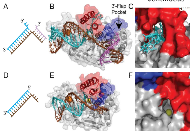
Figure 1. Similarities between 5'-nuclease superfamily members hEXO1-352 and hFEN1-336 in complex with DNA. (A) Double flap and (D) 3'-overhang substrate DNAs crystallized with (B) hFEN1-336 (5UM9) and (E) hEXO1-352 (3QE9). The helical arch ( \alpha 4 - \alpha 5 ) is shown as red and \alpha 2 - \alpha 3 is shown in blue. (C) The exit site of the 5'-flap through the back of arch is shown in close up for hFEN1, with the potential exit site of a flap from hEXO1 also illustrated (F).
