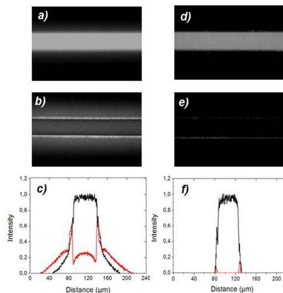
Figure 4. Rhodamine B adsorption and absorption studies. Images a ) and d ) show the absorption of 100 μM Rhodamine B (24 h incubation) in 50 μm wide channels fabricated from PDMS and Flexdym™ respectively. Images b ) and e ) show PDMS and Flexdym™ adsorption and leakage after rinsing with DI water. The corresponding intensity profiles show the normalized fluorescence intensity for PDMS and Flexdym™ in c ) and f ) respectively (black and red lines correspond to 24 h incubation and after rinsing, respectively).
