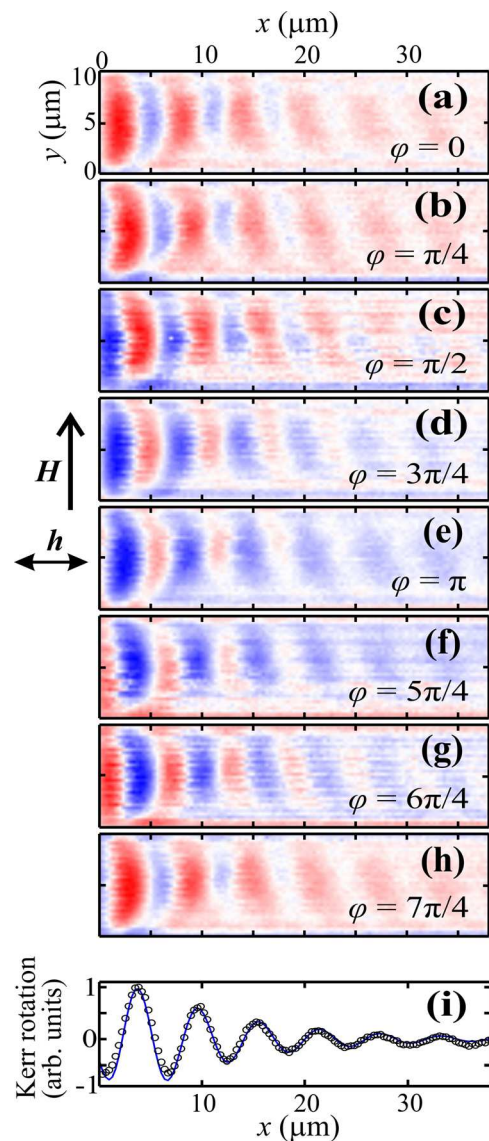
FIG. 2. (a)–(h) Kerr images of the dynamic magnetization are shown for the excitation at 6.24 GHz in phase \varphi (time) steps of \pi/4 (22 ps). (i) The black circles and blue solid line show the Kerr signal from panel (b) averaged over the middle part of the stripe's width ( y = 5 \pm 2.5 \mu\text{m} ) and its fit to an exponentially decaying harmonic function, respectively.
