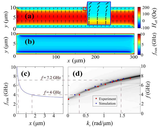
FIG. 4. (a) The calculated projection of the static effective field onto the magnetization in the ground magnetic state is shown with the color scale for the 100 nm thick permalloy stripe of finite length. The unit vectors (averaged over 205 \times 410 mesh cells) show the orientation of the relaxed magnetization. (b) The calculated spatial distribution of f_{\text{FMR}}(\mathbf{r}) calculated using Eq. (1) is shown for the state from panel (a). (c) A cross-section of the f_{\text{FMR}}(\mathbf{r}) along the length of the stripe is shown for the first 5 \mu\text{m} from its left end and y = 5 \mu\text{m} . (d) The spin-wave dispersion calculated from the simulations of an infinitely long stripe is shown by the grayscale, with the overlaid red circles and blue diamonds, showing the points deduced from the measurements and simulations of the finite-length stripes, respectively. For the dispersion calculation, the results of the simulations were spatially smoothed so as to mimic the experimental resolution. The horizontal dashed lines extending from panels (c) to (d) illustrate the correspondence between the source region and wave number of propagating spin waves excited at frequencies of 4 and 7.2 GHz.
