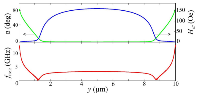
FIG. 5. The top panel shows the numerically simulated coordinate dependence of the angle \alpha between the static magnetization and the y -axis and of the projection of the total internal field H_{\text{eff}} on the direction of the static magnetization in the infinite stripe. The bottom panel shows the corresponding distribution of the local FMR frequency f_{\text{FMR}} calculated from the same simulations using Eqs. (1) and (2).
