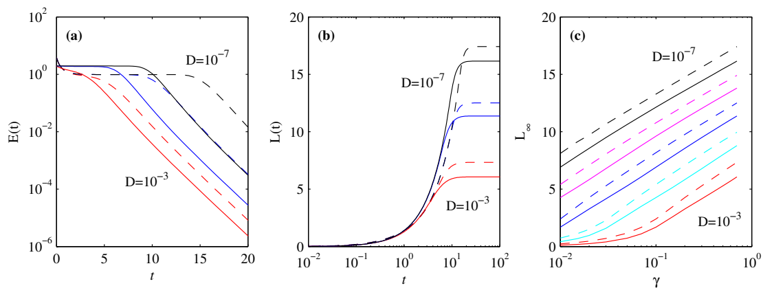
Figure 5. (a,b) show \mathcal{E} and \mathcal{L} , respectively, as functions of time, for \gamma = 0.7 ; (c) shows \mathcal{L}_\infty as a function of \gamma . All three panels are for FP only. The solid lines are the on-quenching process considered here; the dashed lines are for the off-quenching process considered in [40]. D = 10^{-3} to 10^{-7} as indicated. Note the different combinations of linear and logarithmic scales to emphasize different features in different quantities.
