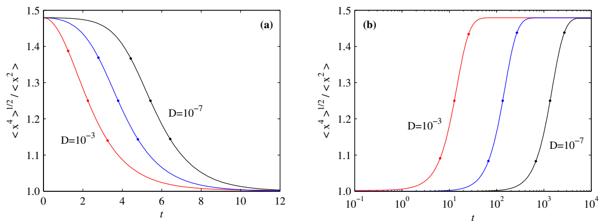
Figure 1. The ratio \sqrt{\langle x^4 \rangle} / \langle x^2 \rangle as a function of t , for the three values D = 10^{-3} (red), 10^{-5} (blue) and 10^{-7} (black). (a) shows FP with t on a linear scale; (b) shows BP with t on a logarithmic scale. All six curves are for \gamma = 0.7 . The three dots on each curve correspond to the solutions shown in Figures 2 and 3. The central dot is always when \sqrt{\langle x^4 \rangle} / \langle x^2 \rangle = 1.25 . In (a), the other two dots are at t \pm 1 relative to the central one; in (b), they are at t/2 and 2t relative to the central one.
