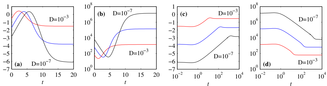
Figure 7. (a) Entropy S(t) for FP; (b) Fisher information I(t) for FP; (c) entropy S(t) for BP; (d) Fisher information I(t) for BP. Note how S and I are essentially opposites of each other. Again also note how the equilibration time scale is O(\ln D^{-1}) for FP, and O(D^{-1/2}) for BP.
