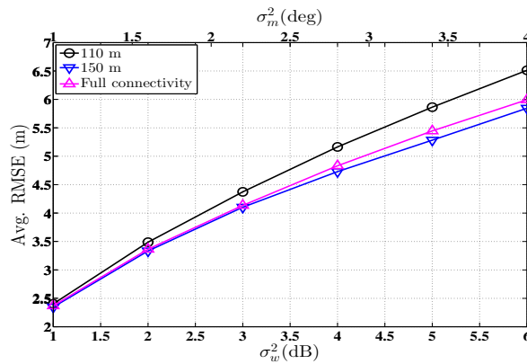
Figure 9. Performance comparison for LLS-Coop AoA-RSS model with partial connectivity. RSSs set 1, \sigma_{w_{ij}}^2 = \sigma_{w_{jk}}^2 = \sigma_w^2 , \sigma_{m_{ij}}^2 = \sigma_{m_{jk}}^2 = \sigma_m^2 , v = 1500 , \alpha_i \forall i = 2.5 .
