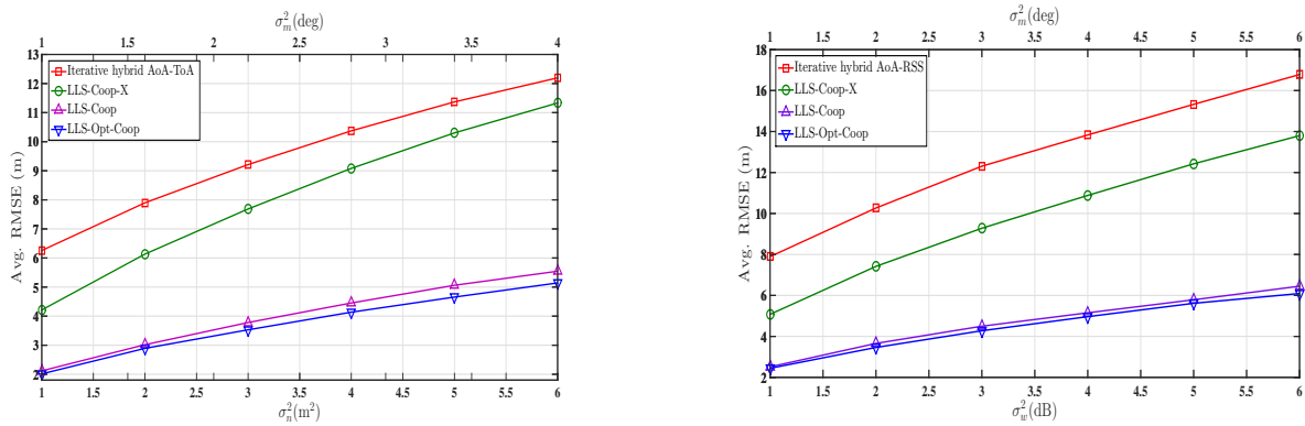
(a) Performance comparison for AoA-ToA signal model. RSs set 2, v = 1000 . (b) Performance comparison for AoA-RSS signal model. RSs set 2, v = 1000 , \alpha_i \forall i = 2.5 .
