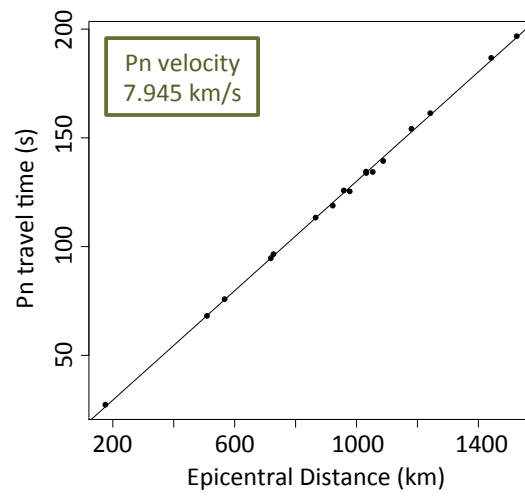
Figure 2: Travel time of the Pn seismic phase from the MBL earthquake to POLNET stations (black circles) as a function of epicentral distance. Linear regression yields an average Pn velocity of \sim 7.95 km/s.
