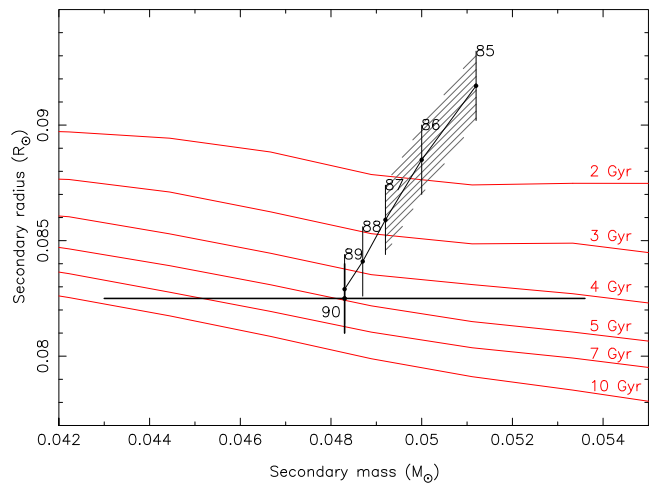
Figure 6. Constraints on the mass and radius of the brown dwarf in SDSS J1205–0242. The black line shows how the mass and radius vary as a function of inclination, given our observational constraints. Note that the radius measurements correspond to the volume-averaged radius of the brown dwarf. Inclinations less than 85^\circ are ruled out, as the brown dwarf would fill its Roche lobe. The hatched region shows the inclinations excluded by the secondary eclipse data. Also shown in red are theoretical mass–radius relationships for solar metallicity brown dwarfs of different ages (Baraffe et al. 2003). The uncertainty on the brown dwarf’s mass from the radial velocity data (which dominates over the inclination uncertainty) is shown on the 90^\circ model. The implication of these models is that SDSS J1205–0242 has a total system age between 2.5 and 10 Gyr.
