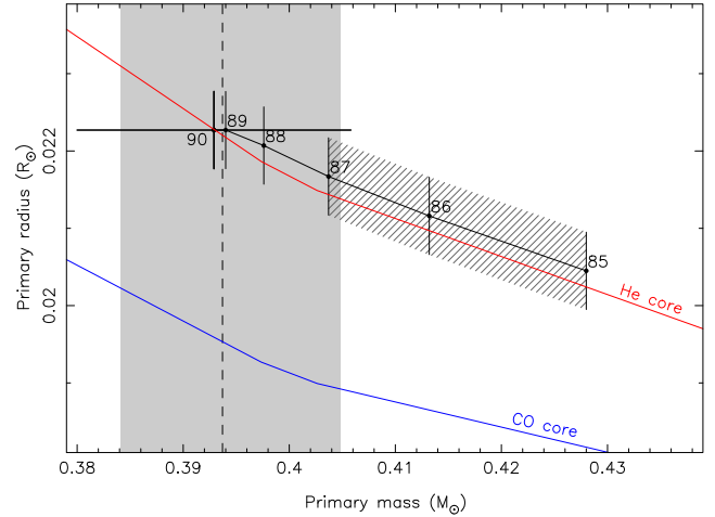
Figure 5. Constraints on the mass and radius of the white dwarf in SDSS J1205–0242 based on our radial velocity and eclipse fitting. The black line shows how the mass and radius vary as a function of inclination. The red line shows the theoretical mass–radius relationship for a 24 000 K helium-core white dwarf with a canonically thick surface hydrogen layer (Panei et al. 2007). The blue line shows the same theoretical mass–radius relationship but for a carbon–oxygen core white dwarf (Fontaine, Brassard & Bergeron 2001), also with a canonically thick surface hydrogen layer. The vertical dashed line marks the white dwarf mass as determined from the Balmer-line fits to our SOAR spectrum, with the shaded area showing the 1\sigma uncertainties on this fit. The hatched region shows the inclinations excluded by the secondary eclipse data. The uncertainty on the white dwarf’s mass from the radial velocity data is shown on the 90^\circ model.
