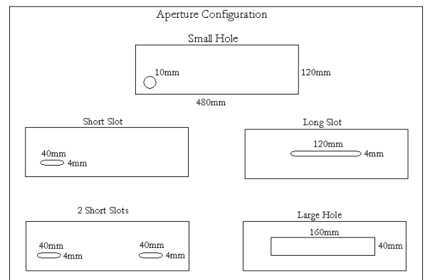
Figure 1: Aperture Configuration used on the front panel of the EUT to provide differing levels of shielding. Also used was a “No holes” configuration with all apertures sealed. These configurations provide the 6 points in Figure 5.
