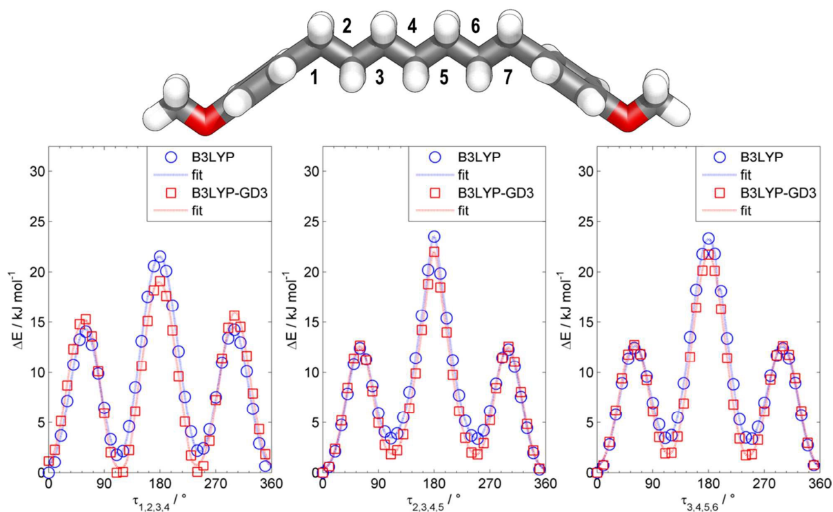
Figure 6: Plots of energy ( \text{kJ mol}^{-1} ) vs dihedral angle ( \tau_{1,2,3,4} , \tau_{2,3,4,5} and \tau_{3,4,5,6} ) obtained using the B3LYP level of DFT (blue circles) and at the B3LYP-GD3 level of DFT (red squares) with the 6-31G(d) basis set. Fits to the values are shown for guidance.
