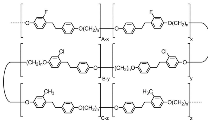
Figure 7: Structures of copolymers reported by Ungar et al. that exhibit nematic to nematic phase transitions (denoted as N-N 2 in the text), where n is equal to 5, 7 or 9. 57
