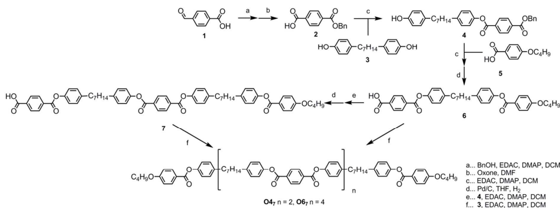
Figure 2: The synthesis of O4 7 and O6 7
