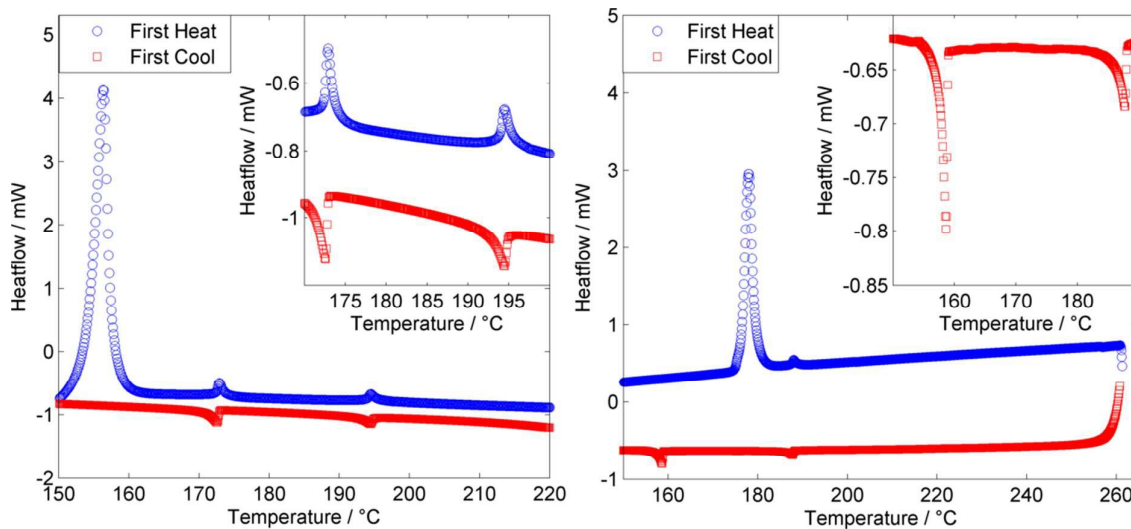
Figure 4: DSC thermograms for O4 7 with an expansion of the region between 170-200 °C (left) and for O6 7 with an expansion of the region between 150-190 °C (right). Both thermograms were obtained using a heat/cool rate of 10 °C min -1 .
