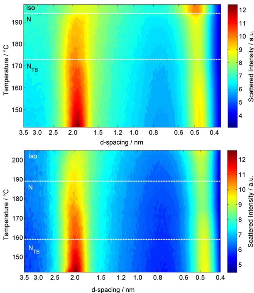
Figure 5: Contour plots of variable temperature small angle X-ray scattering (VT-SAXS) of the tetramer O4 7 (top) and the hexamer O6 7 (bottom).
