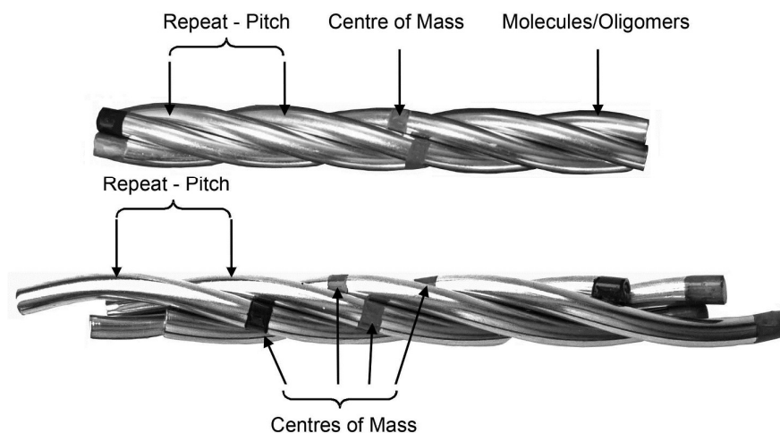
Figure 9: Schematic of the twisted fibre model of the N_{TB} phase, shown with commensurate (top) and incommensurate (bottom) centres of mass.
