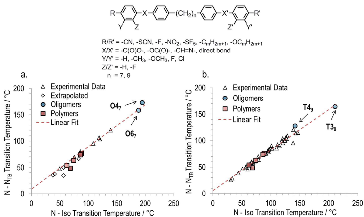
Figure 8: The general structure of 'two-ring' mesogenic dimers and bimesogens with various terminal groups, lateral groups and ring-ring linking groups with heptamethylene and nonamethylene spacers that provided data for plots of the T_{NTB-N} versus the T_{N-Iso} for dimers, bimesogens and oligomers with (a) heptamethylene spacers and (b) nonamethylene spacers. Linear fits, given by equations 1 and 2 in the text, correspond to data for pure bimesogens only ( i.e. oligomers, polymers and extrapolated values were excluded from the fit, but were found to be in good agreement). In cases where differing transition temperatures were reported (CB7CB, CB9CB)
