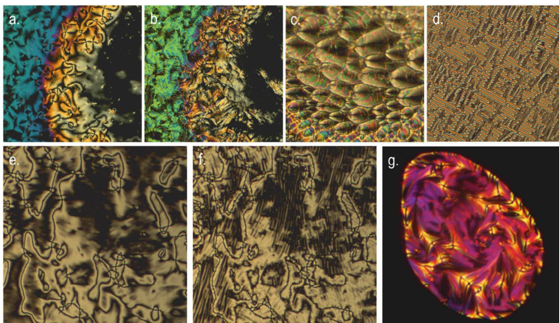
Figure 3: Photomicrographs (x100, crossed polars) of: (a) the schlieren texture and a homeotropic region of the nematic phase of O4 7 at 184 °C on an untreated glass slide; (b) the same region cooled into the N_{\text{TB}} phase of O4 7 at 169 °C showing the 'blocky' texture and a homeotropic region; (c) parabolic defects in an uncovered droplet of the N_{\text{TB}} phase phase exhibited by O4 7 at 166 °C; (d) the rope-like texture of the N_{\text{TB}} phase of O4 7 observed in a 5 \mu\text{m} cell treated for planar alignment at 128 °C; (e) the schlieren texture of the nematic phase of O6 7 at 174 °C on an untreated glass slide; (f) approximately the same region of O6 7 cooled into the N_{\text{TB}} phase at 156 °C showing the blocky texture; (g) a different region of the same slide showing numerous focal conic defects present alongside the blocky texture of the N_{\text{TB}} phase of O6 7 at 147 °C. We note that, qualitatively, these textures are almost identical with those exhibited by the dimers.
