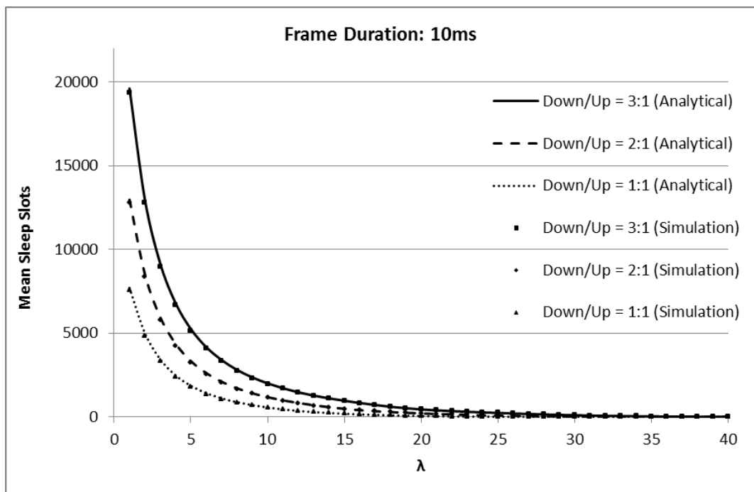
Fig. 5 Mean number of sleep slots per downlink sub-frame as a function of the mean number of requested slots \lambda , for 10ms long frame.
