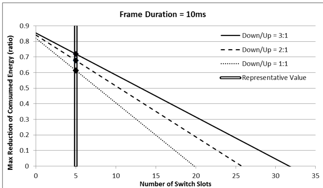
Fig. 9 Maximum reduction of consumed energy (expressed as ratio) as a function of the number of switch slots, for 10ms long frame.
