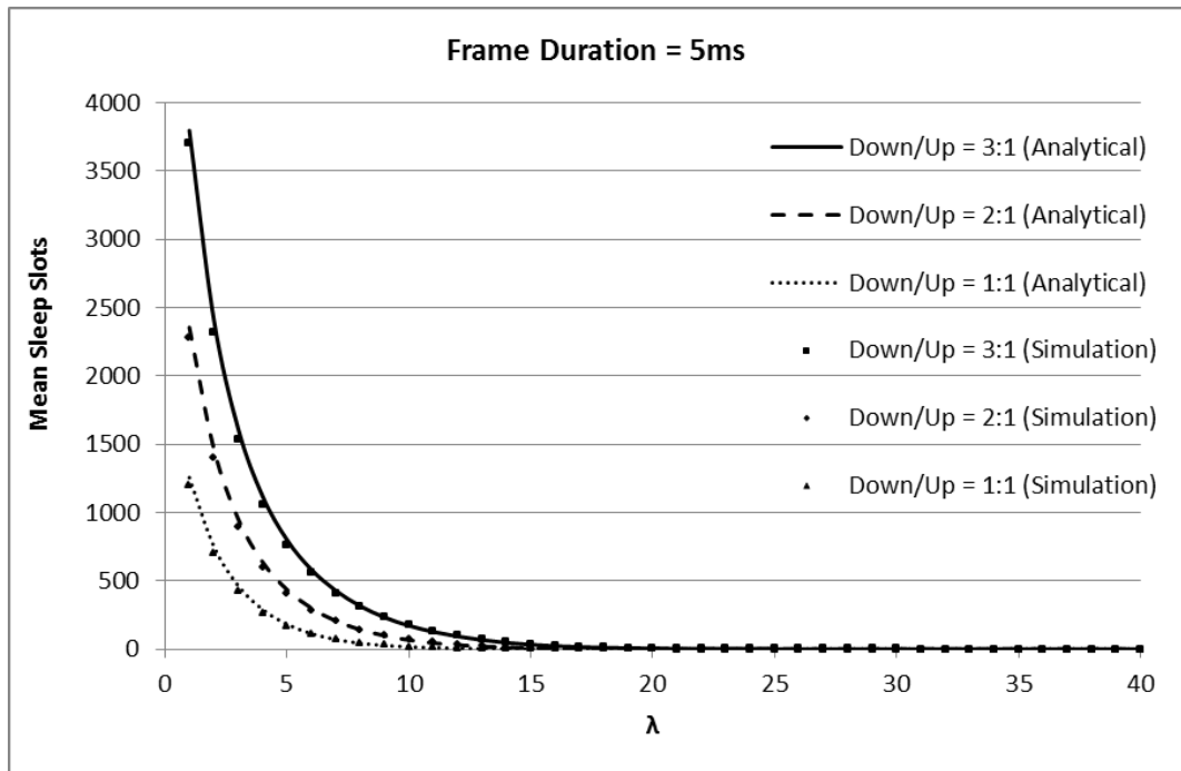
Fig. 4 Mean number of sleep slots per downlink sub-frame as a function of the mean number of requested slots \lambda , for 5ms long frame.
