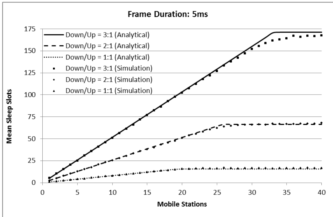
Fig. 6 Mean number of sleep slots per downlink sub-frame as a function of the number of subscriber stations, for 5ms long frame.
