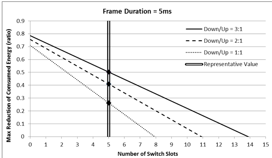
Fig. 8 Maximum reduction of consumed energy (expressed as ratio) as a function of the number of switch slots, for 5ms long frame.
