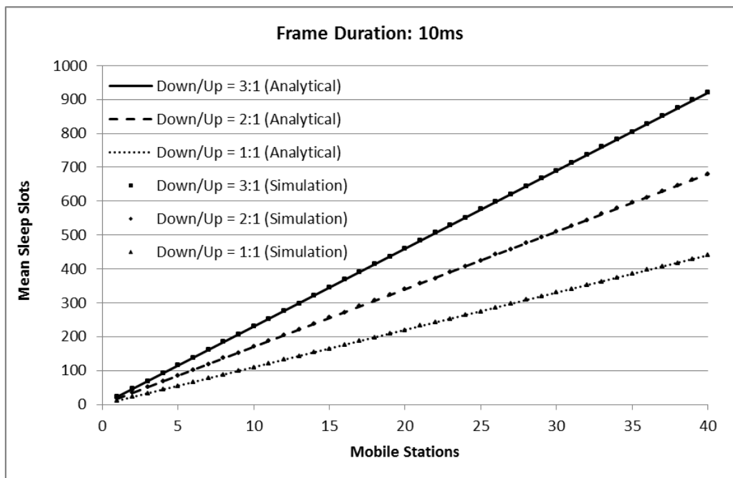
Fig. 7 Mean number of sleep slots per downlink sub-frame as a function of the number of subscriber stations, for 10ms long frame.
