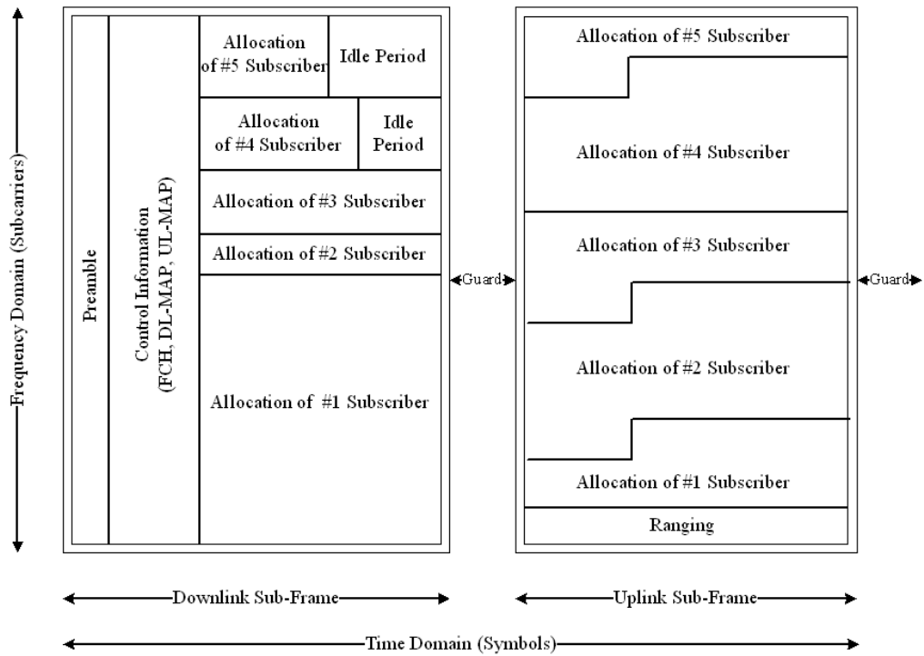
Fig. 1 The IEEE 802.16 TDD frame structure.
