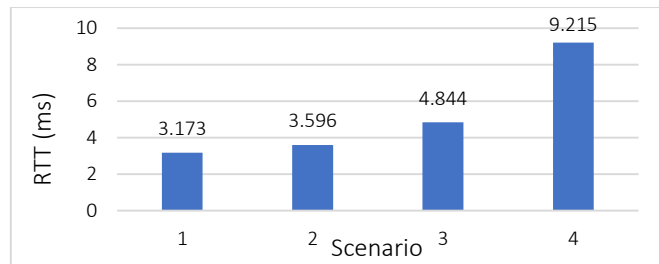
Fig. 6. Average Round Trip Time (RTT) using batctl-ping
