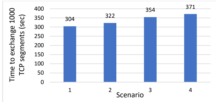
Fig. 7. Time required to exchange 1000 TCP segments using custom socket-based tool
