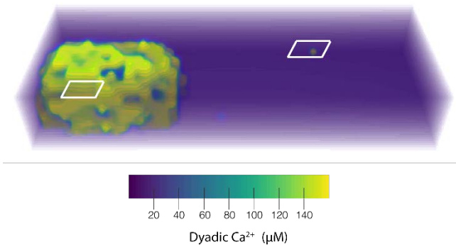
Figure 5. \text{Ca}^{2+} wave and \text{Ca}^{2+} spark originating at sites of MCU block. Areas highlighted are sites of MCU block.
