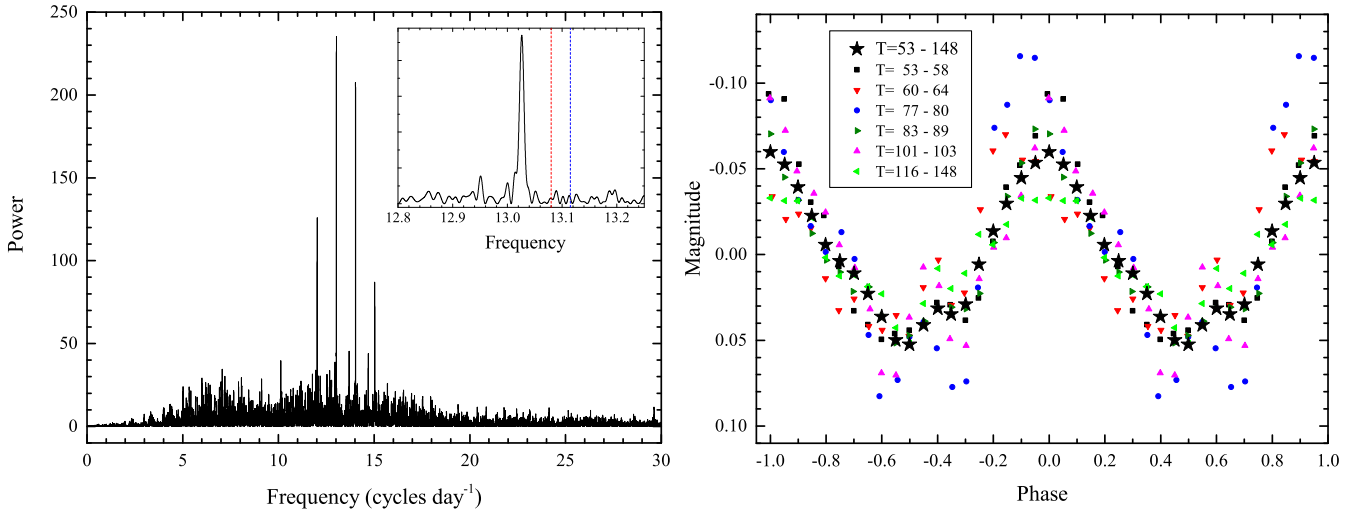
Figure 10. Left: Lomb–Scargle periodogram of the V data combined between T = 53 and 148. The inset shows the enlarged region around the frequency 13.026 \text{ cycle d}^{-1} – the frequency of post-superoutburst modulations observed in 2013. The vertical dashed lines mark the orbital (blue) and stage B superhump (red) frequencies of 13.11 and 13.08 \text{ cycle d}^{-1} , respectively. Right: the entire set (large stars) and short subsets (small symbols) of the V data between T = 53 and 148, folded according to ephemeris HJD_{\text{max}} = 245\,6300.0610(3) + 0.076\,768\,87(5)E .
