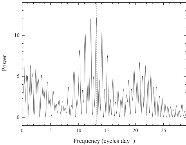
Figure 15. Lomb–Scargle periodogram for spectral data of SSS J122222 obtained during the T = 28 – 30 time interval. The vertical dashed line marks the orbital frequency of 13.112 cycle \text{d}^{-1} .
