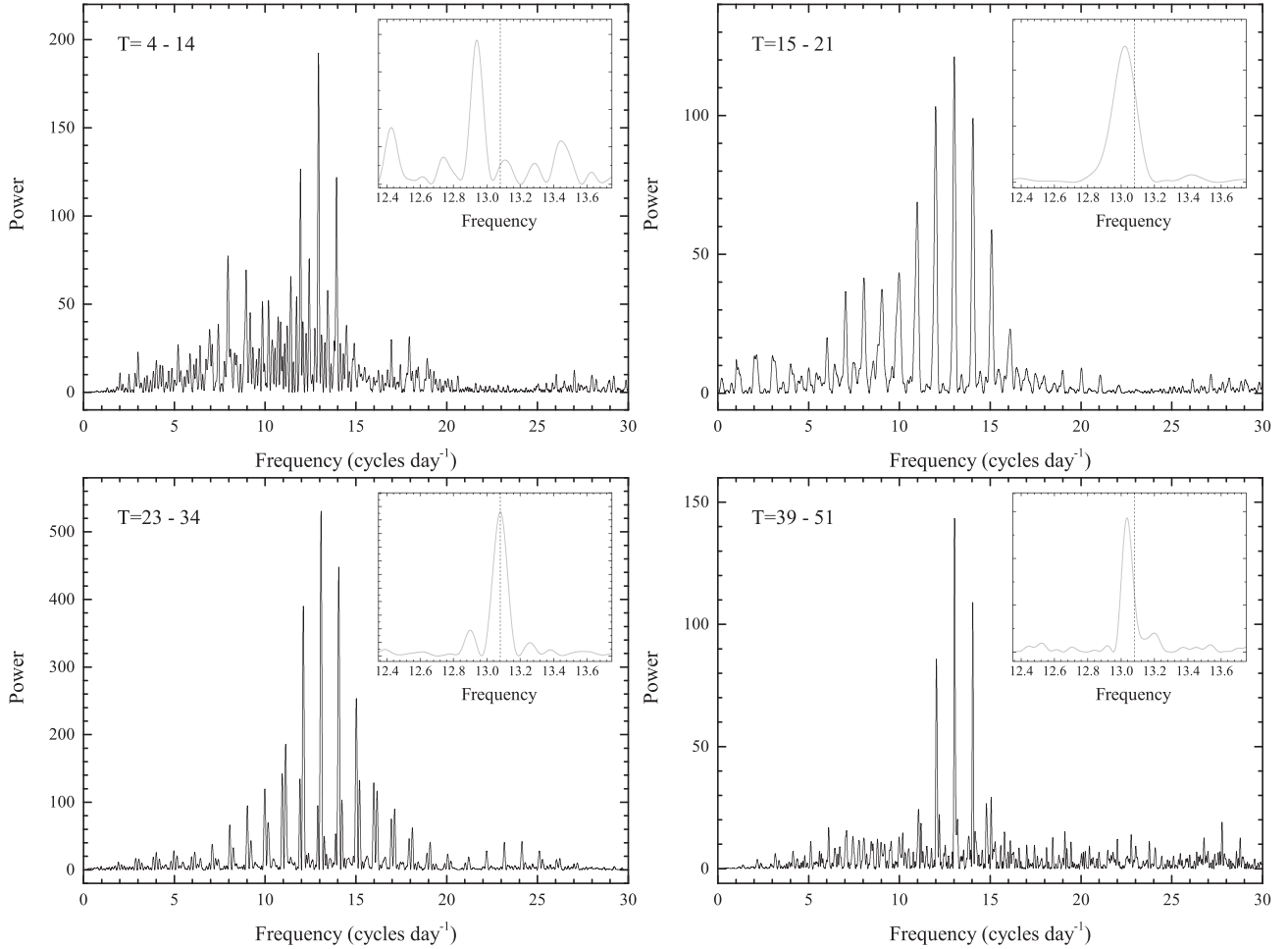
Figure 7. Lomb–Scargle periodograms of the V data combined among T = 4\text{--}14 , 15\text{--}21 , 23\text{--}34 and 39\text{--}51 . The inset shows the enlarged region around the frequency 13.08\text{ cycle day}^{-1} – the averaged frequency of superhumps during the superoutburst stage B, marked by the vertical dashed line.
