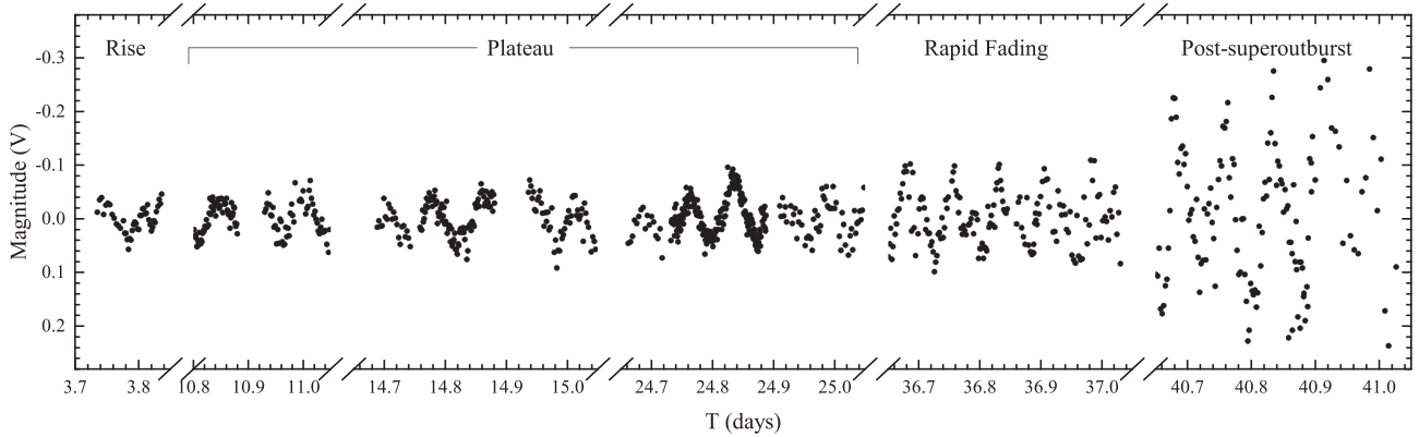
Figure 5. Six light-curve samples from different stages of the superoutburst of SSS J122222 (with the means and linear trends subtracted for each night).
