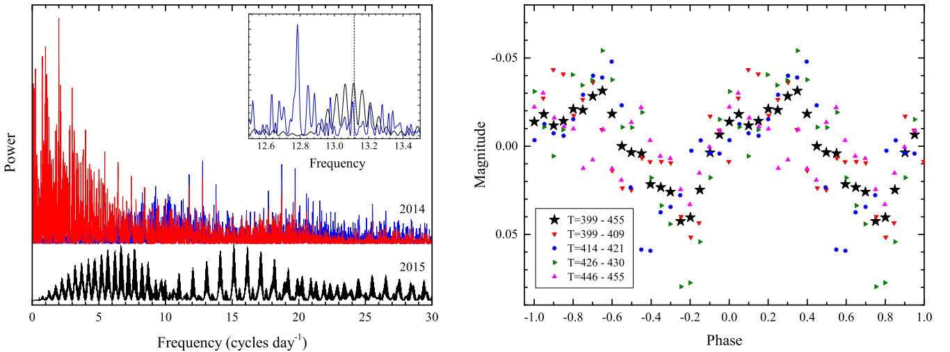
Figure 11. Left: Lomb–Scargle power spectra for optical data of SSS J122222 obtained in 2014 ( T = 399\text{--}455 , two upper spectra) and 2015 ( T = 740\text{--}763 , a bottom spectrum). The red line represents the spectrum for the original 2014 photometry, whereas the blue and black lines are for the detrended data. The inset shows the enlarged region around the orbital frequency marked by the vertical dashed line. Right: the entire set (large stars) and short subsets (small symbols) of the detrended data, obtained in 2014 and folded with the period of 112.6 min.
