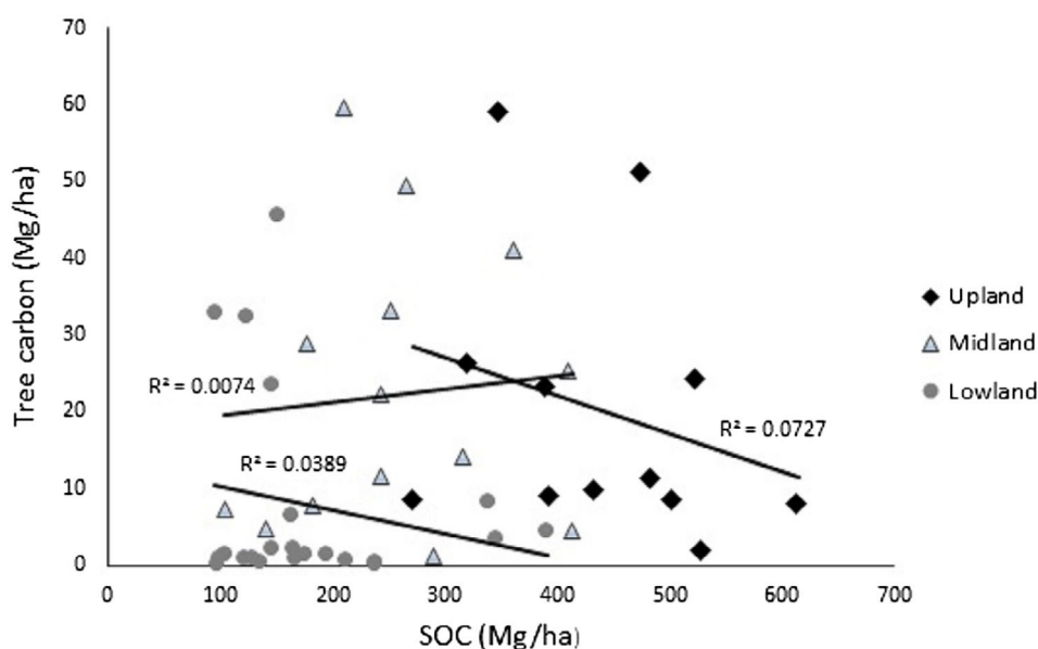
Figure 4. Scatter matrix of SOC and tree carbon showing their relation across the land use zones.
