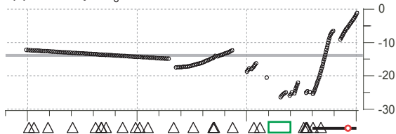
(a) best fit Bpeat \delta^{14}\text{C} 14C WMD
