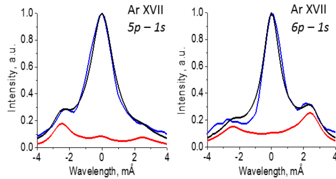
Figure 6. Ar XVII \text{He}\delta and \epsilon profiles obtained at J-KAREN at I_L=3 \cdot 10^{18} \text{ Wcm}^{-2} . The blue lines are for the experimental profiles, the solid red lines for the theoretical profiles from a bi-chromatic region and the solid black lines for the total theoretical profiles including a region of no-periodic-field. The black lines exhibit satellites at 2\omega_L .
