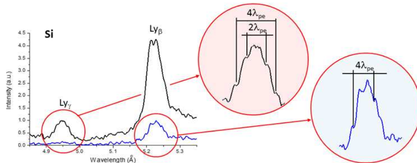
Figure 2. Observation of the Langmuir dips in \text{Ly}\beta (blue trace) and \text{Ly}\gamma (black trace) corresponding to different incident laser irradiances 0.24 \cdot 10^{21} \text{ Wcm}^{-2} (blue trace) and 1.01 \cdot 10^{21} \text{ Wcm}^{-2} (black trace).
