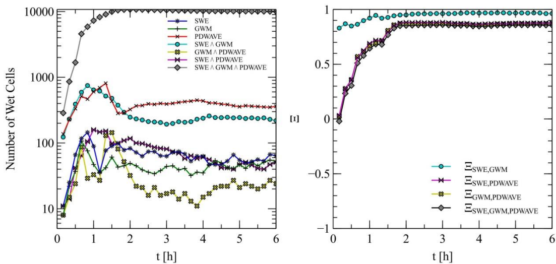
Figure 10 - Left: Number of wet cells in time for each model and each combination of models. Right: \Xi_m Coefficient comparing all combinations of models.
