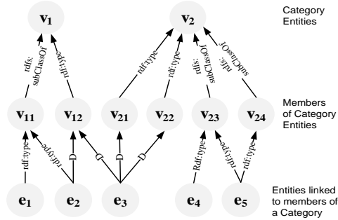
Fig. 1. A data graph showing entities and relationship types between entities.
