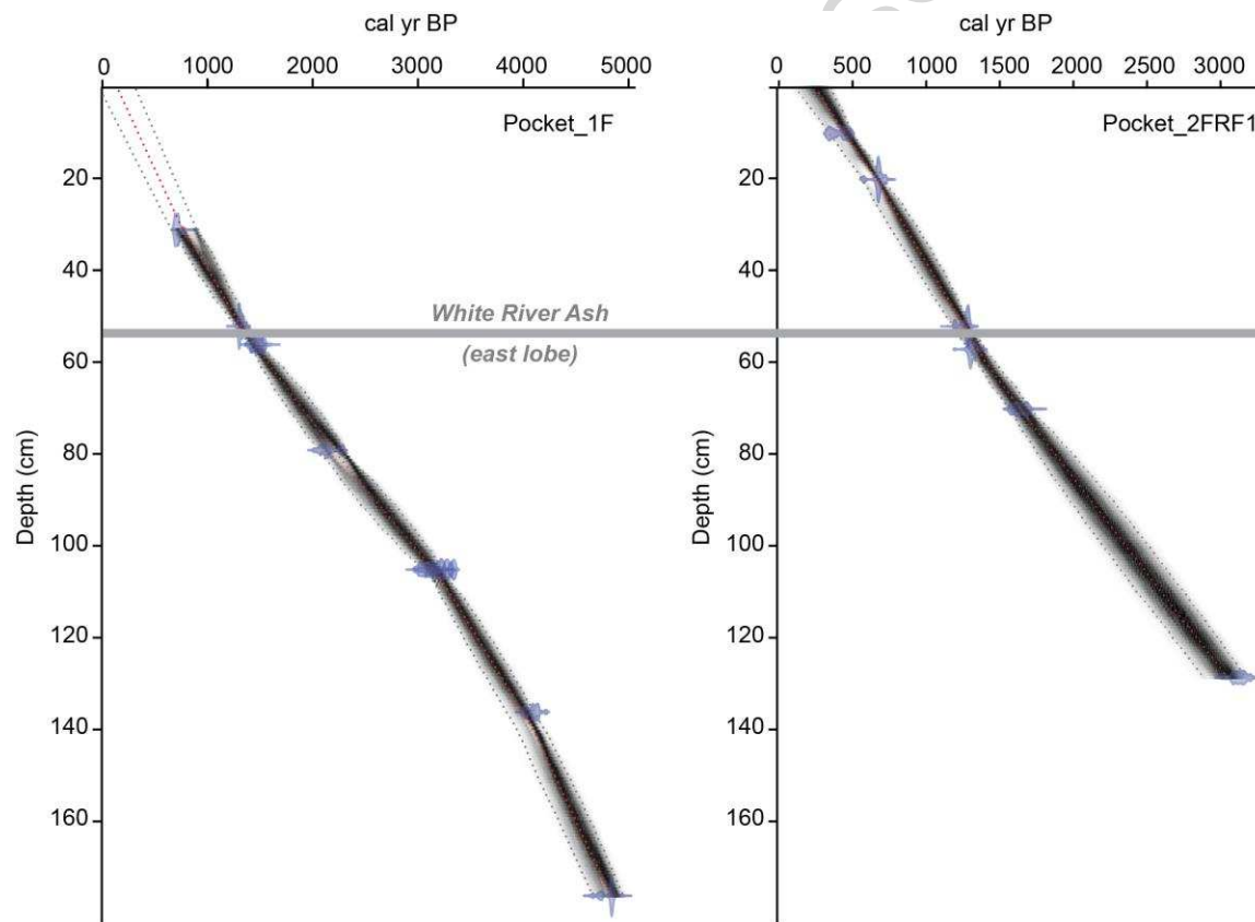
Figure 4. Age-depth models from the two Pocket Lake cores showing the depth of the White River Ash ( 1110 \pm 50 cal BP) and the projected surface ages. Models were created using Bacon v2.2 (Blaauw and Christen 2011) and the IntCal13 calibration curve (Reimer et al., 2013)
