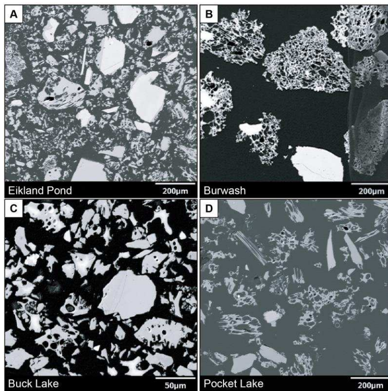
Figure 2. Electron microprobe derived images of glass shards from each site (A. Eikland Pond; B. Burwash; C. Buck Lake; D. Pocket Lake). Both Pocket Lake and Burwash Dune samples are characterized by vesicles with similar properties, and shards displaying a frothy, fibrous and platy morphology. Shards from Pocket Lake were morphologically distinct from the frothy and fibrous shards from Eikland Pond, and the frothy, bubble-walled, stretched and platy tephra from Buck Lake.
