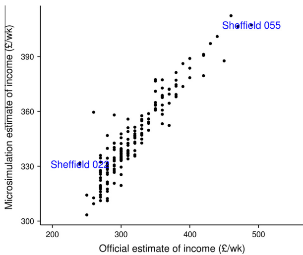
Fig. 9. Scatter graph of mean equivalised household income produced as an output from the spatial microsimulation model (y axis) and official estimates from the Office of National Statistics for the 173 Medium Super Output Areas of South Yorkshire. (Max. and min. official estimates labelled in blue.) (For interpretation of the references to colour in this figure legend, the reader is referred to the web version of this article.)
