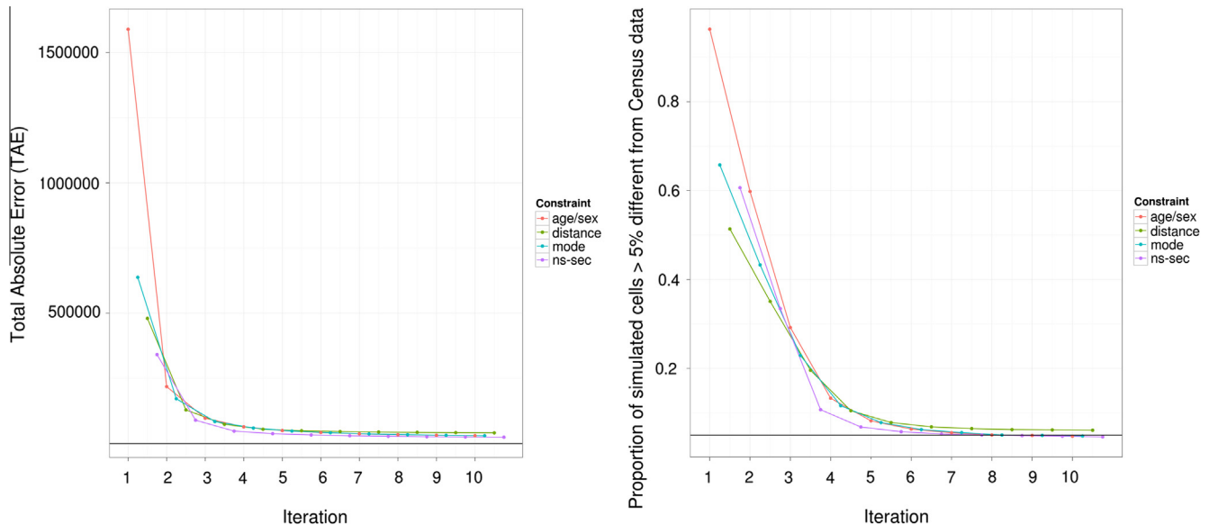
Fig. 2. Improving fit between simulated and census data across all 4 constraint variables outlined in Table 4, as illustrated by decreasing values of the total absolute error (TAE) (left) and decreases in the proportion of simulated aggregate cell values that differ from census data by more than 5% (right) after each constraint and iteration. The horizontal black lines represent 0 error and 5% of cell values, respectively.
