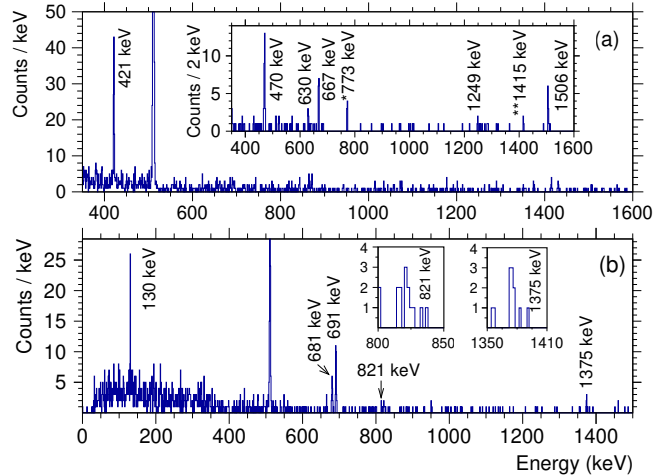
Figure 2: (a) \gamma -rays emitted in prompt coincidence (0-200 ns) following the detection of \beta particles and (inset) \gamma -rays emitted between 0.2 and 4 \mu\text{s} after detection of the \beta particle. The \gamma ray marked with a *773 keV is the 4^+ \rightarrow 2^+ in ^{92}\text{Mo} and is attributed to correlations with the time random background, the 2^+ \rightarrow 0^+ (transition not labeled) is also present at 1510 keV, the **1415 keV is the decay from the 2^+ \rightarrow 0^+ in the granddaughter ^{96}\text{Pd} . (b) \gamma -rays emitted in prompt coincidence following the detection of a \beta delayed proton (insets left and right show the 821 keV and 1375 keV transitions, respectively). In both cases the decay events are uniquely correlated to the previous ^{96}\text{Cd} ion implanted in the same pixel, using the method discussed in section 2, and using a \beta correlation time of 1.35 s, which is three half lives of the 16^+ isomer deduced in the current work.
