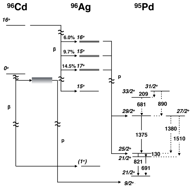
Figure 3: Proposed decay scheme for the \beta decay and \beta p decay of the 16^+ isomer in ^{96}\text{Cd} , the transitions marked with dashed lines were not observed but are within the available angular momentum of the proton decay. The calculated branching ratios to the GT resonance states in ^{96}\text{Ag} , extracted from LSSM calculations, are also presented. The partial decay scheme of ^{95}\text{Pd} was taken from [11]
