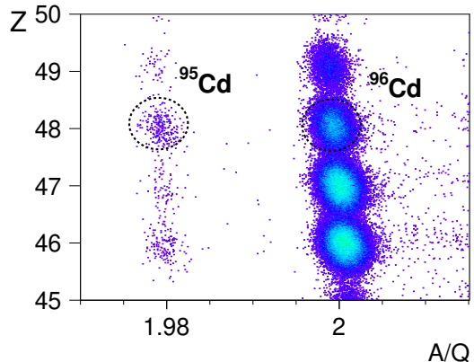
Figure 1: The particle ID for ions transmitted through BigRIPS and identified as being implanted in the active stopper (AS).
