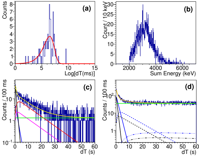
Figure 4: (a) Sum of natural \log(dT) for all \beta - and \beta p -delayed \gamma -rays observed after the decay of the 16^+ spin gap isomer in ^{96}\text{Cd} , where dT is the time between a correlated implant and decay event. The red line is the result of a fit using the Schmit method which yields a mean lifetime (halflife) of 649_{-58}^{+72} \text{ ms} ( 450_{-43}^{+53} \text{ ms} ), (b) Sum energy recorded in the active stopper SIMBA, for \beta -delayed proton events in coincidence with ^{96}\text{Cd} implanted ions. (c) Time distributions of \beta -delayed proton events in coincidence with ^{96}\text{Cd} ions. All implantation events found within a time window of 60 s prior to the decay were correlated. The fit result is shown in yellow, the individual components, parent ( ^{96}\text{Cd}(16^+) ): black, ^{96}\text{Cd}(0^+) : blue), daughter ( ^{96}\text{Ag}(8^+) : pink, ^{96}\text{Ag}(2^+) : red), background (green), are also shown. (d) same as (c) except for \beta -decay events, the fit result is shown in yellow, the individual parents are solid lines ( ^{96}\text{Cd}(16^+) : black, ^{96}\text{Cd}(0^+) : blue), daughters are dashed lines ( ^{96}\text{Ag}(8^+) : black, ^{96}\text{Ag}(2^+) : blue), and granddaughters are dot-dashed lines ( ^{96}\text{Pd}(0^+) : black/blue).
