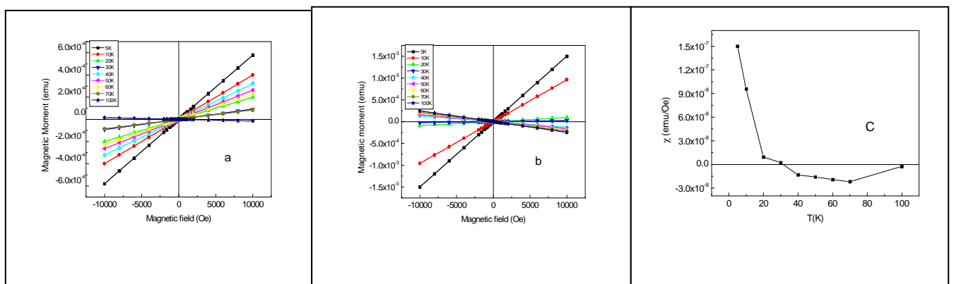
Fig. 4 (Colour on line) The subtracted susceptibility of the films (a) on the SrTiO 3 substrate (b) on the LaAlO 3 substrate and (c) the high field susceptibility for the film on the LaAlO 3 substrate.
