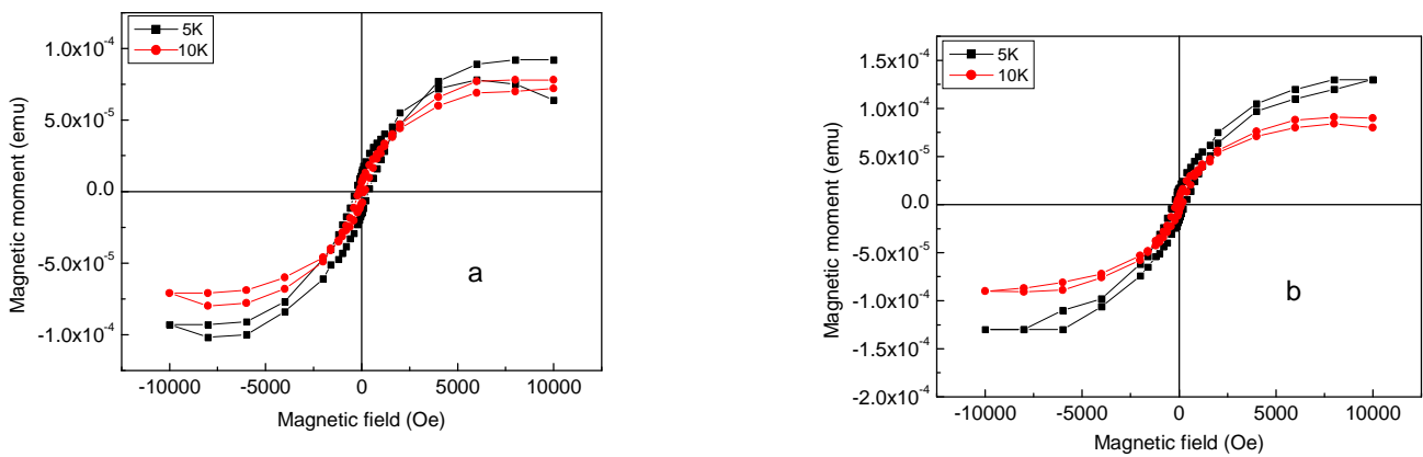
Fig. 3 (Colour on line) The hysteresis loops for the field in plane (with linear background subtracted) at temperatures 5K and 10K for the films on (a) SrTiO 3 and (b) LaAlO 3 substrates.
