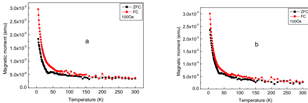
Fig. 2 (Colour on line) Field cooled and zero field cooled data taken in an in-plane field of 100Oe for films of GdMnO 3 on (a) SrTiO 3 and (b) LaAlO 3 substrates. The data for the bare substrates has been subtracted.
