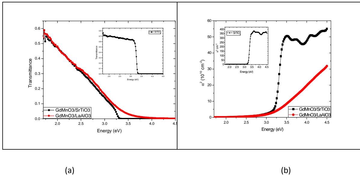
Fig. 5(Colour on line) (a) Transmittance (b) the absorption \alpha squared for the two films. The SrTiO 3 substrate absorbs strongly above 3.2eV and its spectra are shown in the inserts.
