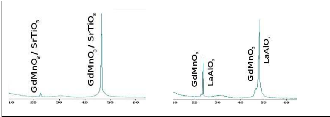
Fig.1 Xray data from films of GdMnO 3 on the SrTiO 3 and LaAlO 3 substrates showing epitaxy.
