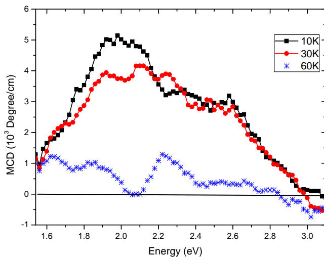
Fig. 7 The MCD spectrum taken at remanence for \text{GdMnO}_3 on \text{SrTiO}_3 there is a finite spectrum at 10\text{K} and 30\text{K} , the spectrum at 60\text{K} is almost zero. The remanent spectra for a blank substrate (which was anyway very small, < 0.1 ) has been subtracted from this data.
