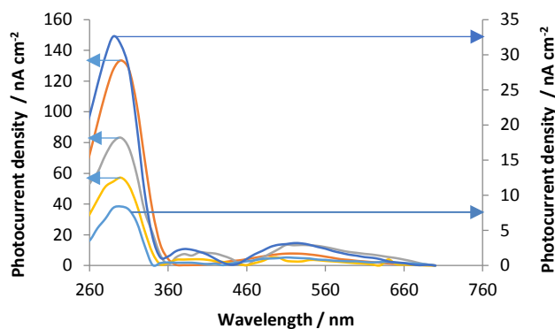
Figure 10: Photocurrent response from a series of devices functionalised with \text{Ru(dcbpy)}_2\text{Cl}_2 showing some limited photocurrent in the visible region.
