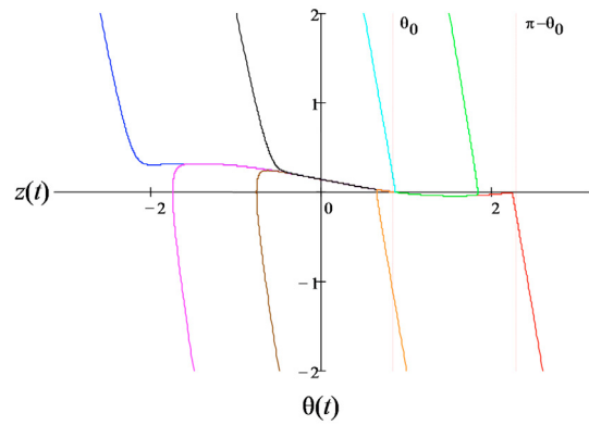
Figure 1. Simulation results for the system (6) with d(t) = 0 and for several arbitrarily chosen initial conditions
