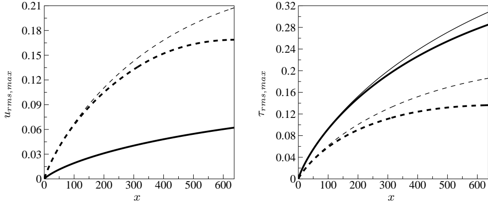
Figure 9: Evolution of the maximum r.m.s. of the streamwise velocity and the temperature for different free-stream Mach number: M_\infty=2 (dashed lines), M_\infty=6 (solid lines). The turbulence Reynolds number is Re_t=4.8 (refer to table 1(c)). Thick lines: nonlinear solutions, thin lines: linearized solution.
