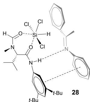
Figure 14. Previously reported model for Sigamide 28 illustrating dual activation.
