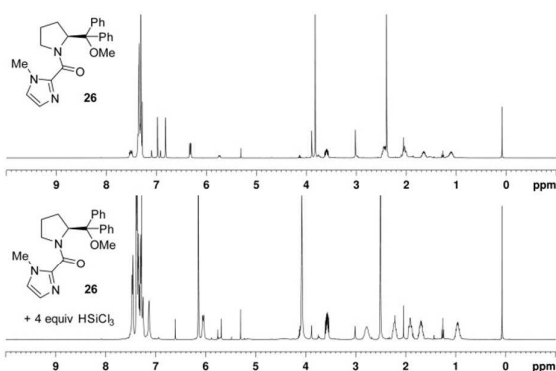
Figure 9. ^1\text{H} NMR spectrum of catalyst 26 before and after addition of 4 equiv HSiCl 3 .
