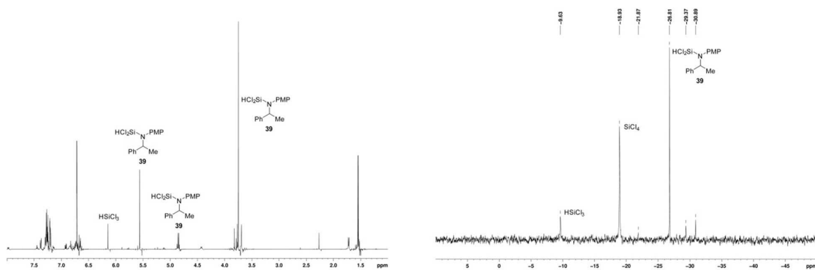
Figure 7. In situ ^1\text{H} and ^{29}\text{Si} NMR spectra of reaction products as depicted in Scheme 1 with catalyst 17 .
