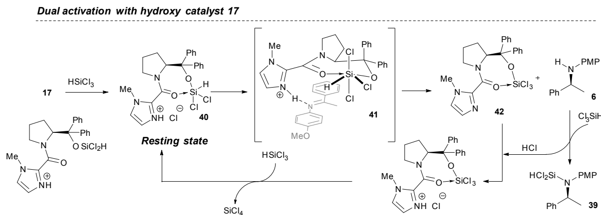
Figure 12. Proposed dual activation mechanism for catalyst 17 .
