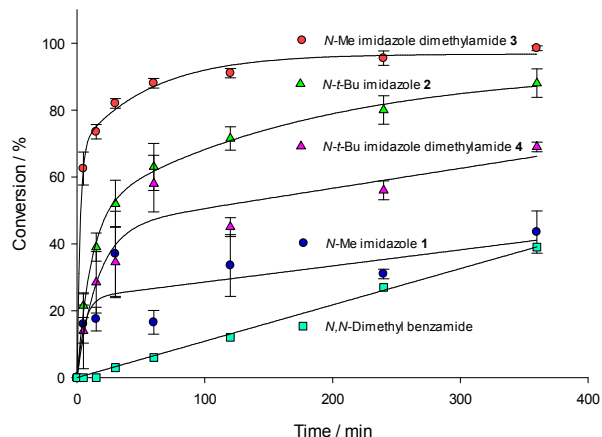
Figure 1. Relative reaction rates of imidazole catalysts 1–4 and N,N -dimethyl benzamide. Reactions performed using 10 mol% catalyst, 2 equiv \text{HSiCl}_3 in DCM ( 1 \text{ mL mmol}^{-1} ) at 0^\circ\text{C} . Conversion calculated from comparison of appropriate integrals in ^1\text{H NMR} spectrum of aliquots removed from reaction.
