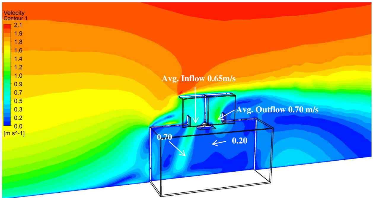
Fig. 6. Air velocity contours in windcatcher without ASCD (up) and with 30° ASCD (down).
