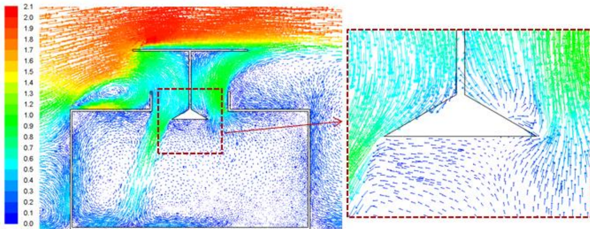
(b) windcatcher with 30° ASCD
