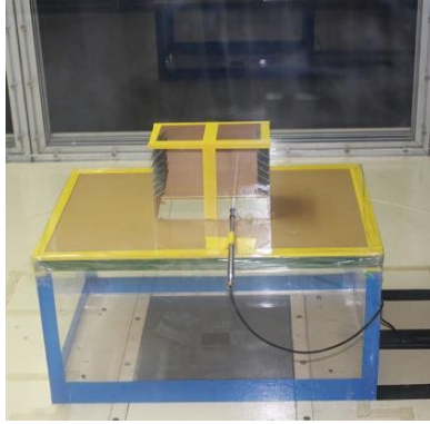
Figure 4. conventional windcatcher (CTSW) model during airflow measurements.
