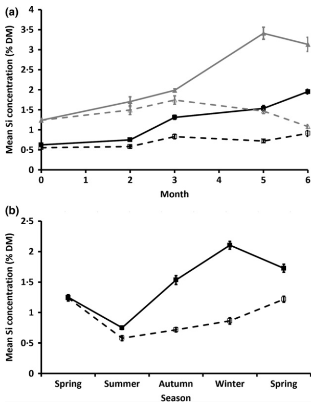
Fig. 1. Induction of silicon defences in Deschampsia caespitosa exposed to high (c. 20% of leaves damaged) and low (c. 5% of leaves damaged) levels of grazing by field voles ( Microtus agrestis ). Solid lines denote high grazing intensity, and broken lines denote low grazing intensity. (a) Comparison of silicon induction in D. caespitosa grown in glasshouse and grazed in the laboratory (grey lines, triangular symbols) (reproduced from Reynolds et al. 2012) and under field conditions (black lines, square symbols) in open grazing enclosures in northern England from May to November 2009 with a grazing intensity of 300 voles \text{ha}^{-1} and 50 voles \text{ha}^{-1} (J. DeGabriel, S. Hartley, F. Massey, S. Reidinger and X. Lambin, unpublished data). (b) Seasonal variation in silicon concentrations in D. caespitosa in field grazing enclosures under high (300 voles \text{ha}^{-1} ) and low (50 voles \text{ha}^{-1} ) grazing treatments from March 2009 to April 2010. Error bars represent standard error.
