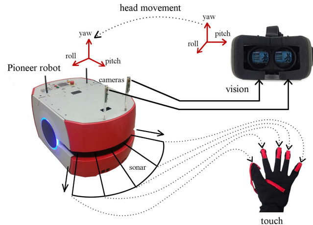
Fig. 9. Mobile robot Pioneer LX used to test the capability of our wearable interface to communicate and control different robotic platforms. Vision was connected to two cameras mounted on the top of the mobile robot. Touch was connected to the integrated front sonar. The human was able to explore a remote environment by receiving multisensory feedback, and controlling the robot movements in various directions, e.g., forward, backward, left and right.
