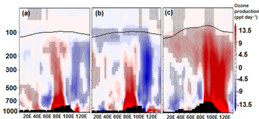
Figure 3. Longitude–pressure cross section of changes in net ozone production ( \text{ppt day}^{-1} ) due to enhanced NO x with respect to the CTRL simulation, averaged for the monsoon season (June–September) obtained from (a) Ind38 (averaged over 8–35° N), (b) Ind73 (averaged over 8–35° N), and (c) Chin73 (over 20–45° N) simulations. The black line shows the tropopause while black hatched lines indicate 95 % confidence level.
