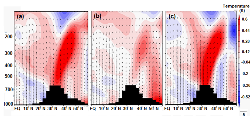
Figure 8. Latitude–pressure cross section of temperature anomalies (K) averaged for the monsoon season (June–September) and over 70\text{--}100^\circ\text{E} obtained from (a) Ind38-CTRL, (b) Ind73-CTRL, and (c) Chin73-CTRL simulations. Black arrows indicate wind vectors (the vertical velocity field has been scaled by 300).
