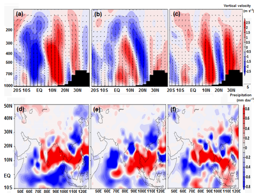
Figure 9. Difference in the meridional circulation due to enhanced NO x emissions averaged for the monsoon season (June–September) and over 70–100° E for (a) Ind38-CTRL, (b) Ind73-CTRL, and (c) Chin73-CTRL simulations. Shaded contours indicate the anomalies in vertical velocity ( \text{m s}^{-1} ). The vertical velocity field has been scaled by 300. Precipitation anomalies ( \text{mm day}^{-1} ) averaged for the monsoon season (June–September) obtained from (d) India38-CTRL, (e) Ind73-CTRL, and (f) Chin73-CTRL simulations.
