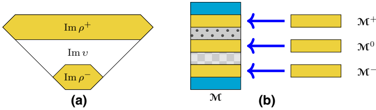
Fig. 2. a The arrangement of image regions \text{Im } \rho^\pm \subset \text{Im } v \subset D_{\mathcal{M}}(\text{Im } \rho^+) used in Lemma 14. b The spacetimes used to compute the cocycle. The map \tilde{\Lambda}_T (resp. \tilde{\Lambda}_S ) is locally constant outside the chequered (resp., dotted ) region
