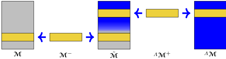
Fig. 1. Diagram of spacetimes involved in constructing \zeta(\tilde{\Lambda})
