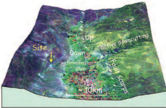
Figure 9 Region around the Taung Valley. A Landsat thematic mapper image (bands 2, 4, and 7 are red, green, and blue respectively) draped over exaggerated digital elevation data to give a 3D effect. An earthquake fault scarp on the east side of the valley is indicated by white arrows. The fault cross-cuts geological features and varies in altitude and thus cannot be a river terrace or other erosional or depositional feature. Uplifting of the eastern flank has caused rivers to incise and the down-dropped valley has been filled with sediment. Faulting may also be associated with the western side of the valley, causing the incised valley that hosted the breccia with the hominin fossil. The down-dropped sedimented basin is today used for agriculture.
