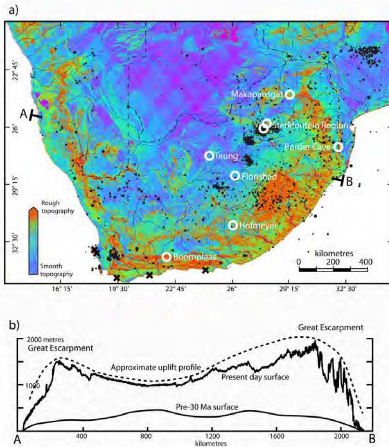
Figure 5 South African topography a) Map of roughness and seismicity as reported by Saunders et al (2008). Roughness is based on SRTM 3 digital elevation data, using an ~18db/octave high-pass filter. In this case the filter emphasizes roughness at horizontal scales less than about 500m. Inland hominin sites are indicated by white circles and coastal sites by black crosses. b) Topographic cross-section along A-B in Figure 5(a). Prior to 30Ma the land surface was smooth and at low altitude similar to much of Australia today. Uplift has been more than 1000m in places.
