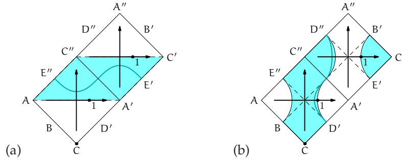
FIGURE 4. Hyperbolic objects in the double cover of \mathbb{R}^h :
