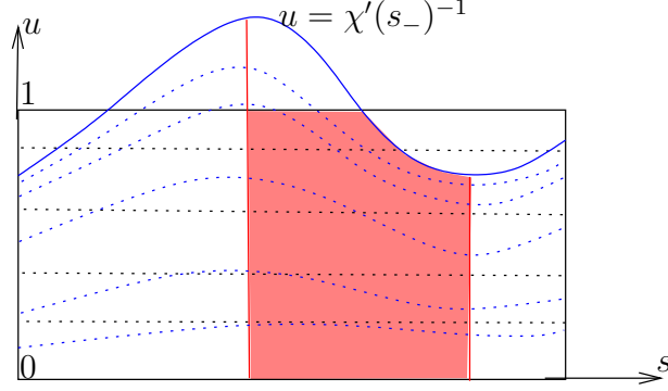
FIGURE 4. Poincaré section.
