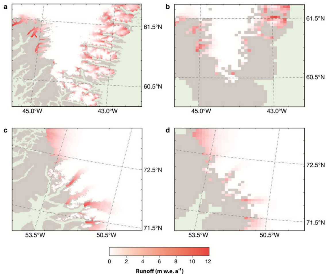
Fig. 4. Mean annual runoff 1990–2010, for specific parts of the south of the GrIS, (a) CS-1 and (b) CS-5, and the mid west of the GrIS, (c) CS-1 and (d) CS-5. Abbreviations as described in Table 1. Grey areas are ice-free land and green areas ocean.
