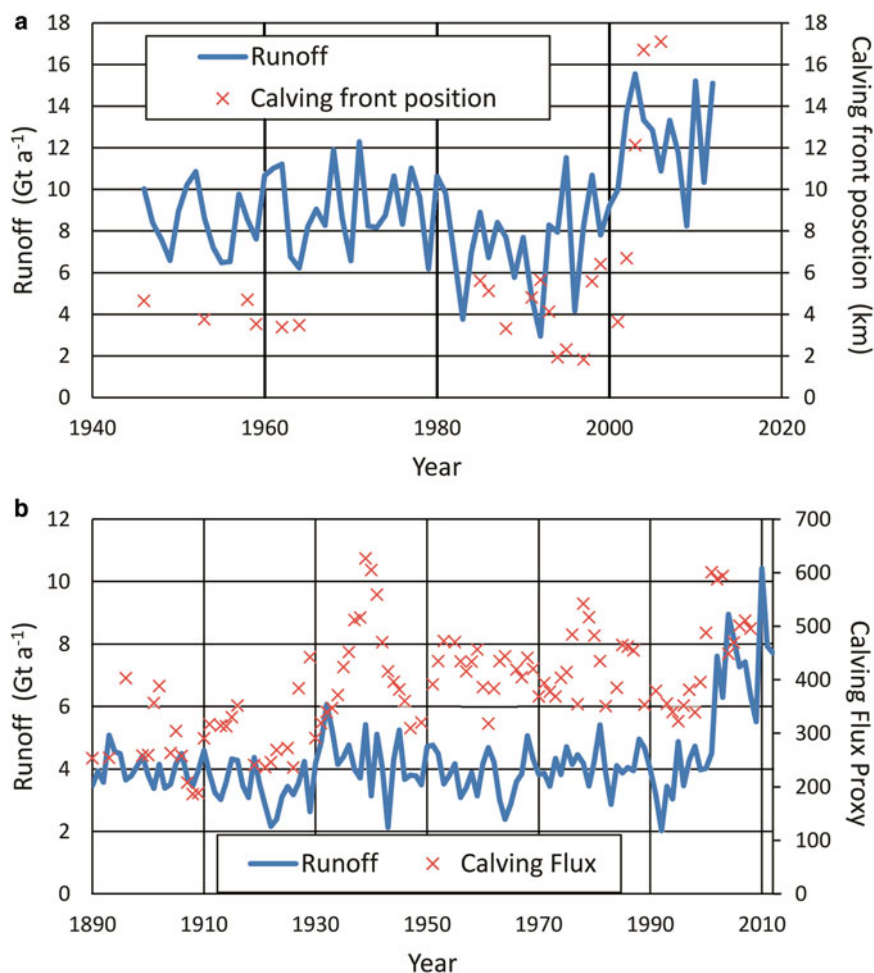
Fig. 11. Correlation between annual runoff and calving data for the areas around specific glaciers, as defined in main text. a) Jakobshavn Isbrae, compared to calving front position measured up glacier, (Csatho and others, 2008), and b) Helheim Glacier compared to calving flux proxy, sand deposition rate ( \text{g m}^{-2} \text{a}^{-1} ) (Andresen and others, 2012).
