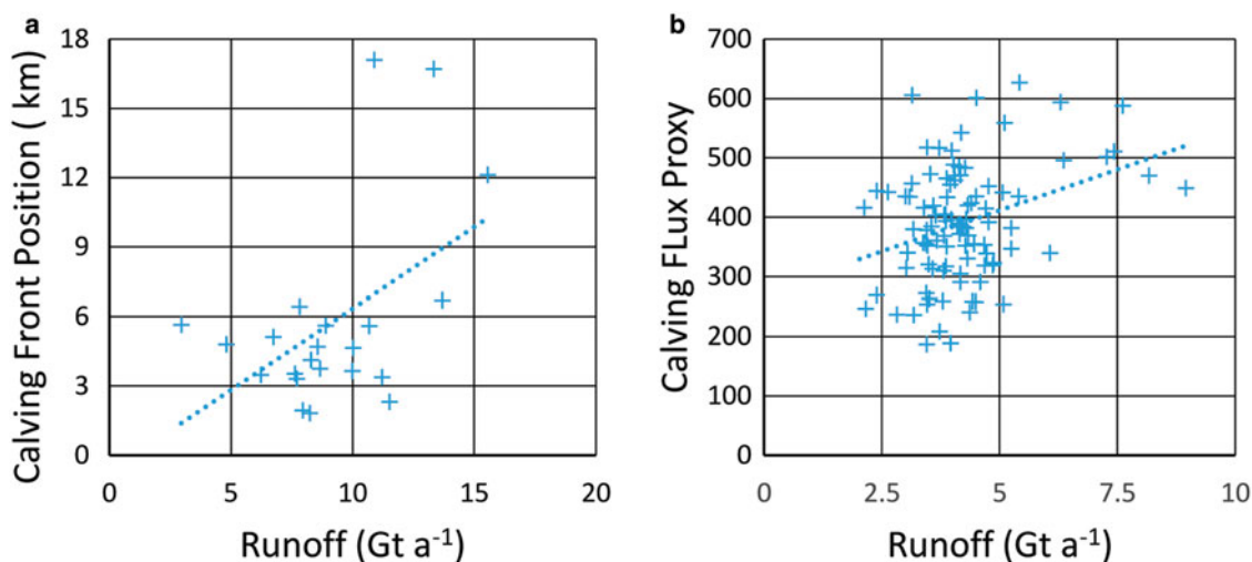
Fig. 12. Scatter plots, with linear trend lines, showing the correlation between annual runoff and calving data for the areas around specific glaciers, as defined in main text. (a) Jakobshavn Isbrae, compared with calving front position (Csatho and others, 2008) and (b) Helheim Glacier, compared with calving flux proxy, sand deposition rate ( \text{g m}^{-2} \text{a}^{-1} ) (Andresen and others, 2012).
