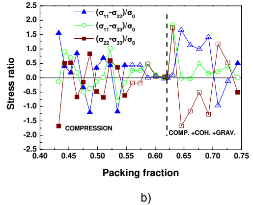
Figure 1: Evolution of the stress tensor with packing fraction in the presence of: a) only gravity and b) gravity and surface energy (1.0 J/m 2 ) were introduced.
