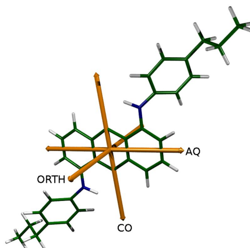
Fig. 12 Carbonyl (CO), anthraquinone (AQ) and orthogonal (ORTH) axes from which the TDM orientations were defined relative to the atoms in the anthraquinone core, shown here with the DFT optimised structure of 15NB3.
