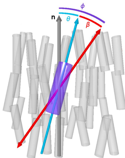
Fig. 1 Schematic representation of a dye molecule (violet cylinder) within the molecules of a nematic liquid crystal host (grey cylinders). The relative orientations of the director, \mathbf{n} (grey arrow), the principal molecular axis of the dye (turquoise arrow) and the TDM of the dye (red arrow) are also shown.
