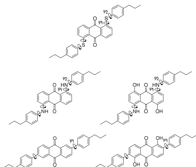
Fig. 10 Structures of the dyes with labels indicating bonds about which the dihedral angle distributions were calculated to have a FWHM > 20^\circ during the guest-host MD simulations.
