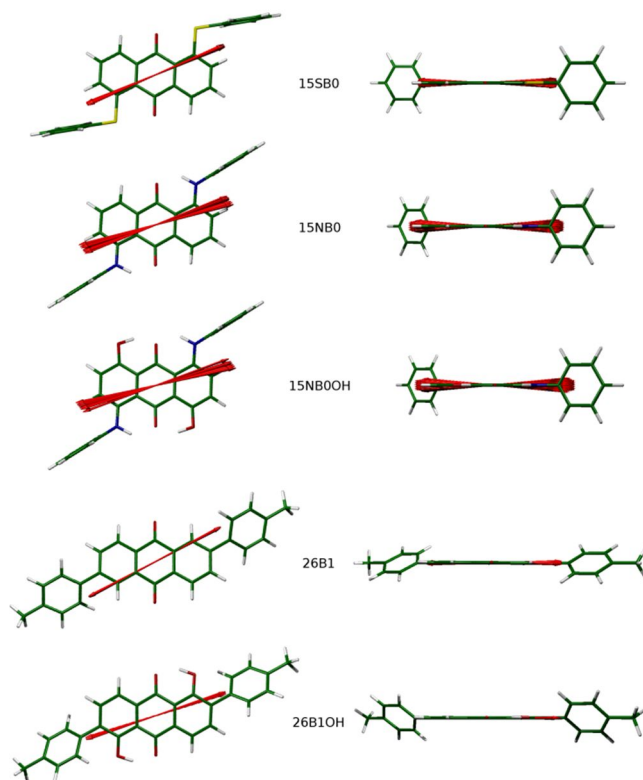
Fig. 13 Model structures corresponding to the most populated dihedral angles of the dyes in the MD simulations, shown approximately perpendicular to the plane of the anthraquinone core (left) and along the anthraquinone carbonyl axes (right). The calculated TDMs from the geometries corresponding to the 95% most populated conformers determined from the MD simulations are overlaid as unit vectors.
