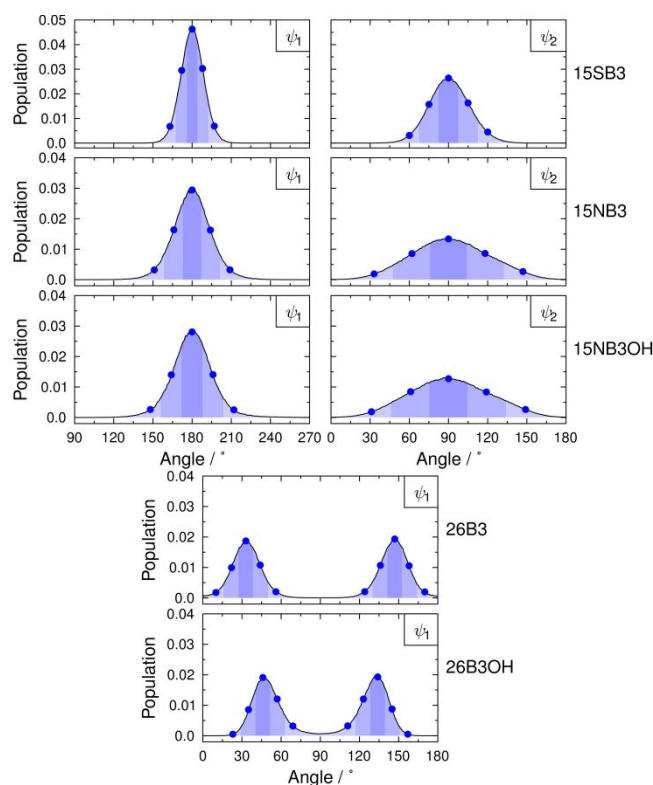
Fig. 11 Dihedral angle population distributions of the dyes from the MD simulations using 1^\circ histogram bin-widths; details described in the Supplementary Information. Blue dots indicate the angles used in the geometries for the TD-DFT calculations of the TDM orientations. Shaded regions indicate the “bins” used to assign geometries from the MD trajectories to those for which the TDM orientations were calculated; the bin ranges are given in the Supplementary Information.
