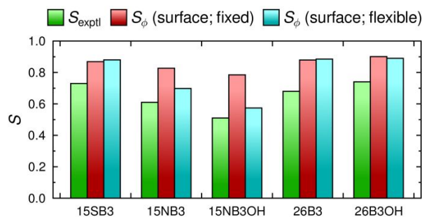
Fig. 14 A comparison of the experimental dichroic order parameters, S_{\text{exptl}} (green), and the calculated values using the surface tensor z -axis as the principal molecular axis with fixed TDM orientations, S_{\phi} (surface; fixed), (red) and variable TDM orientations, S_{\phi} (surface; flexible), (cyan).
