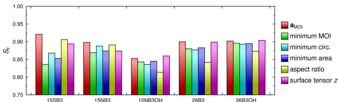
Fig. 5 A comparison of the molecular order parameters of the dyes obtained by using the \mathbf{a}_{\text{MOI}} , minimum MOI, minimum circumference (circ.), minimum area, maximum aspect ratio, and surface tensor z axes.
