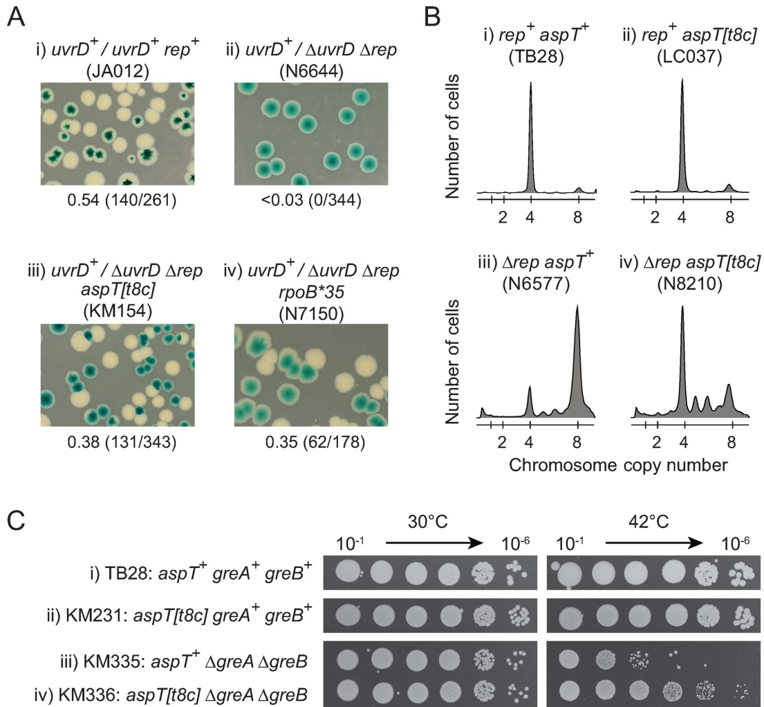
Figure 1. A mutation in an aspartyl tRNA gene suppresses the need for accessory replicative helicases and for anti-backtracking factors. (A) Retention or loss of pRC7uvrD (pAM407) from strains without or with \Delta rep \Delta uvrD deletions as judged by blue/white colony color on LB plates containing X-gal and IPTG. Fractions of white colonies are indicated below each image with actual numbers of white versus total colonies counted in parentheses. (B) DNA content of the indicated strains as monitored by flow cytometry under run out conditions in LB. The number of chromosome equivalents per cell is shown below. (C) The viability of greA^+ greB^+ versus \Delta greA \Delta greB cells without and with aspT[t8c] as monitored by serial dilutions of liquid cultures grown at 30°C and plated subsequently on LB agar at 30°C and 42°C.
