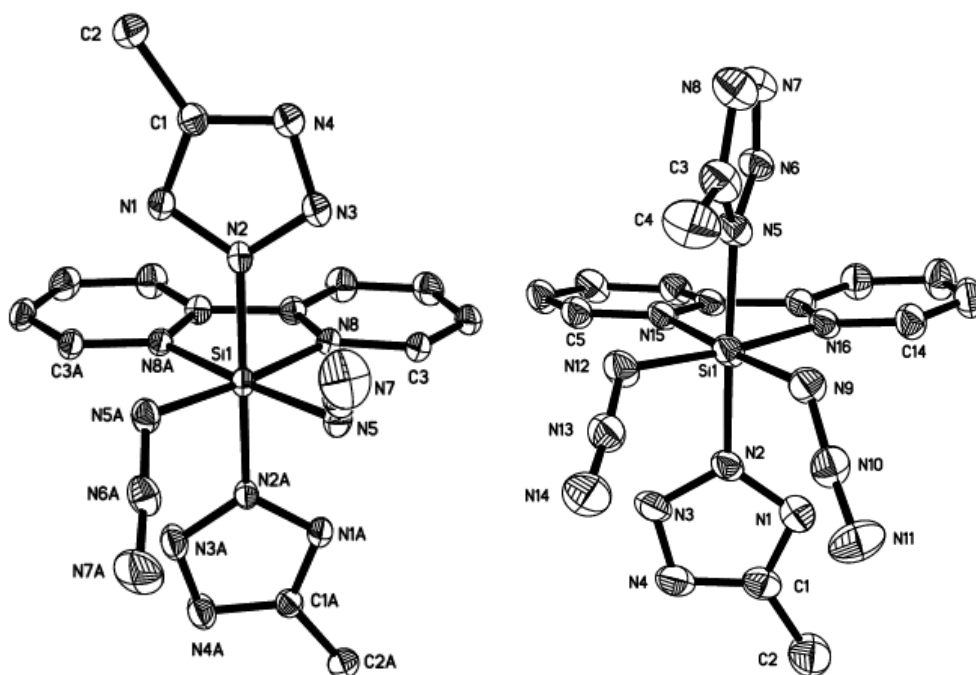
Fig. 2. Thermal ellipsoid plots of OC-6-13 -[Si(N 3 ) 2 (κN(2)-mtz) 2 (bpy)] ( 4a , left) and OC-6-24 -[Si(N 3 ) 2 (κN(1)-mtz)(κN(2)-mtz)(bpy)] co-crystallised with MeCN ( 4b , right) drawn at the 50% probability level. H atoms and MeCN have been omitted for clarity. Selected bond lengths [Å] and angles [°] 4a : Si1-N5 1.804(1), Si1-N2 1.895(1), Si1-N8 1.940(1), N5-N6 1.219(2), N6-N7, 1.137(2), Si1-N5-N6 120.24(9), N5-Si1-N5A 96.42(5); 4b : Si1-N9 1.816(2), Si1-N12 1.802(3), Si1-N2 1.901(3); Si1-N5 1.868(3); N12-N13 1.211(3), N13-N14 1.143(3), N9-N10 1.219(3), N10-N11 1.138(3), Si1-N15 1.944(2), Si1-N16 1.936(3), Si1-N12-N13 123.9(2), Si1-N9-N10 127.3(2), N9-Si1-N12 96.8(1).
