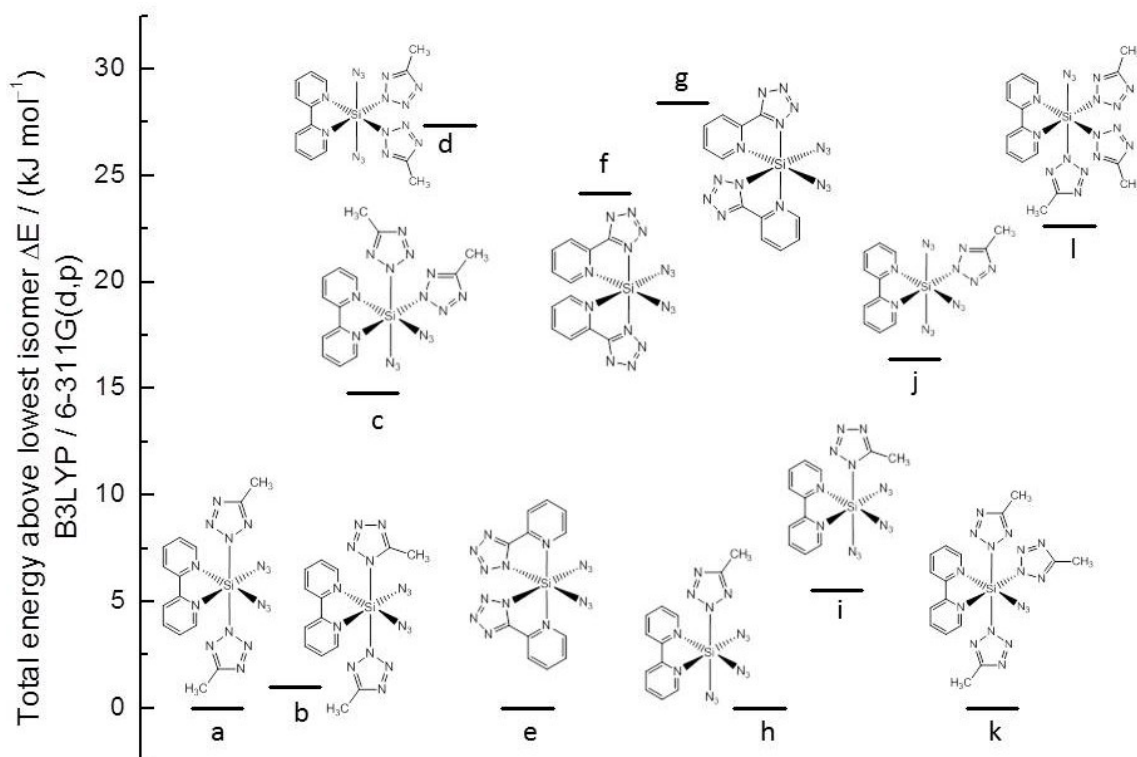
Fig. 5. Total energy differences as calculated by density functional theory at the B3LYP/6-311G(d,p) level of the complexes 4a (a), 4b (b), OC-6-32- (c) and OC-6-33-[Si(N 3 ) 2 ( \kappa N(2)-mtz) 2 (bpy)] (d), 9 OC-6-22- (e), OC-6-13- (f) and OC-6-32-[Si(N 3 ) 2 ( \kappa^2 N,N(1)-pytz) 2 ] (g), OC-6-23-[Si(N 3 ) 3 ( \kappa N(2)-mtz)(bpy)] (h), OC-6-23-[Si(N 3 ) 3 ( \kappa N(1)-mtz)(bpy)] (i) and OC-6-33-[Si(N 3 ) 3 ( \kappa N(2)-mtz)(bpy)] (j), OC-6-31-[Si(N 3 )( \kappa N(2)-mtz) 3 (bpy)] (k) and OC-6-33-[Si(N 3 )( \kappa N(2)-mtz) 3 (bpy)] (l).
