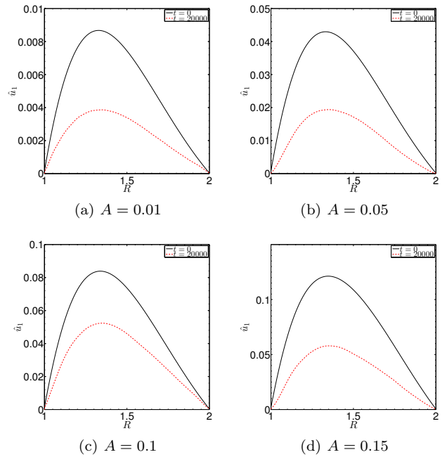
Figure 10. Magnitude of the radial velocity in the m = 1 component of the solution ( |\hat{u}_1| ) as a function of R at the beginning of the simulation (black solid lines; taken from nonlinear secular theory) and at t = 20000 (red dashed lines; representing the end of our simulations). This illustrates the damping of the eccentric mode, and also that its shape remains similar to that predicted by secular theory.
