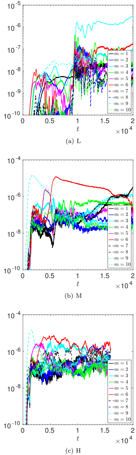
Figure 3. Energy in different azimuthal wavenumber components of the solution ( E_m ) for m \in [1, 10] as a function of time for simulations in a domain with R_o = 2 with c_s = 0.05 and \sigma = 0 for three different resolutions 200 \times 256 (L), 400 \times 512 (M) and 800 \times 1024 (H).
