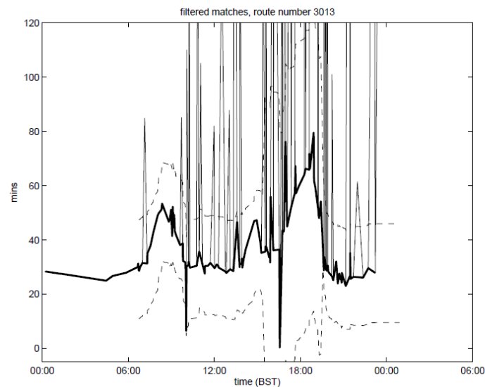
Figure 6: Recovery by detecting lostness then widening the acceptance window.
