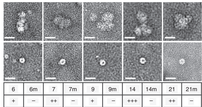
Fig. 4 In vitro pentamer binding to the predicted PSs. In vitro analysis of PS: pentamer interactions by MST, HPeV1 pentamers were titrated into fixed amounts of 5'-Alexa 488-labelled short RNAs encompassing PSs 6, 7, 9, 14 and 21 and their variants (labelled m). The binding data were assessed semi-quantitatively (+/-) noting the amplitude of the signal change over the range of pentamer concentrations and where significant binding began to occur. These were compared to a known PS-CP interaction, that of the 19 nt bacteriophage MS2 TR (translational operator) stem-loop and its CP 40 ( K_d -1-4 nM, depending on binding assay used), which was designated as +++++, i.e. low nano-molar affinity. The highest protein concentration samples from these assays were recovered, negatively-stained and examined by electron microscopy (top row shows the PS and the bottom row shows its mutant). Scale bar is 25 nm
