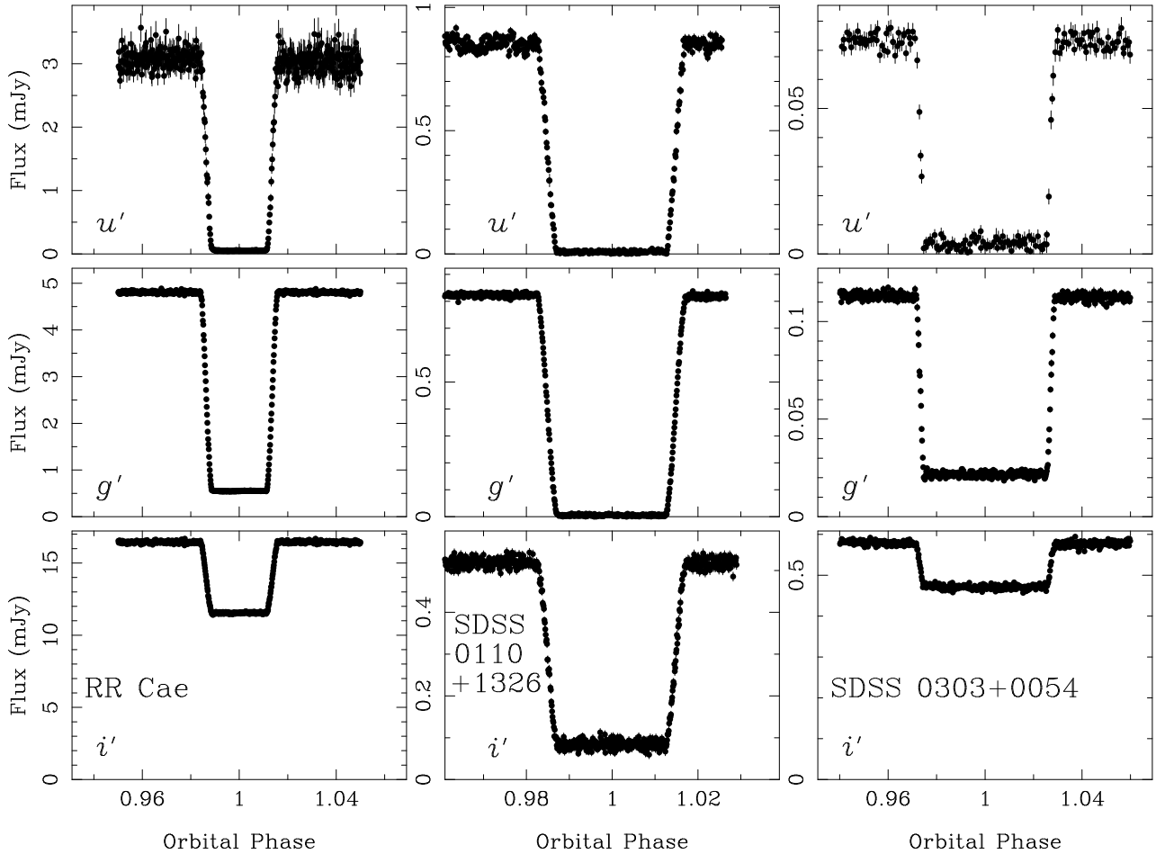
Figure 2. Flux calibrated primary eclipses of (left to right) RR Cae, SDSS 0110 + 1326 and SDSS 0303 + 0054 in (top to bottom) u' band, g' band and i' band. Light curves were made by phase binning all available eclipses then combining them. Any flares were removed before the light curves were combined. Longer exposures were used in the u' band for SDSS 0303 + 0054 since it is very faint in this band. A micro-flare occurs during the ingress of the SDSS 0110 + 1326 eclipse, visible in the u' band light curve.
