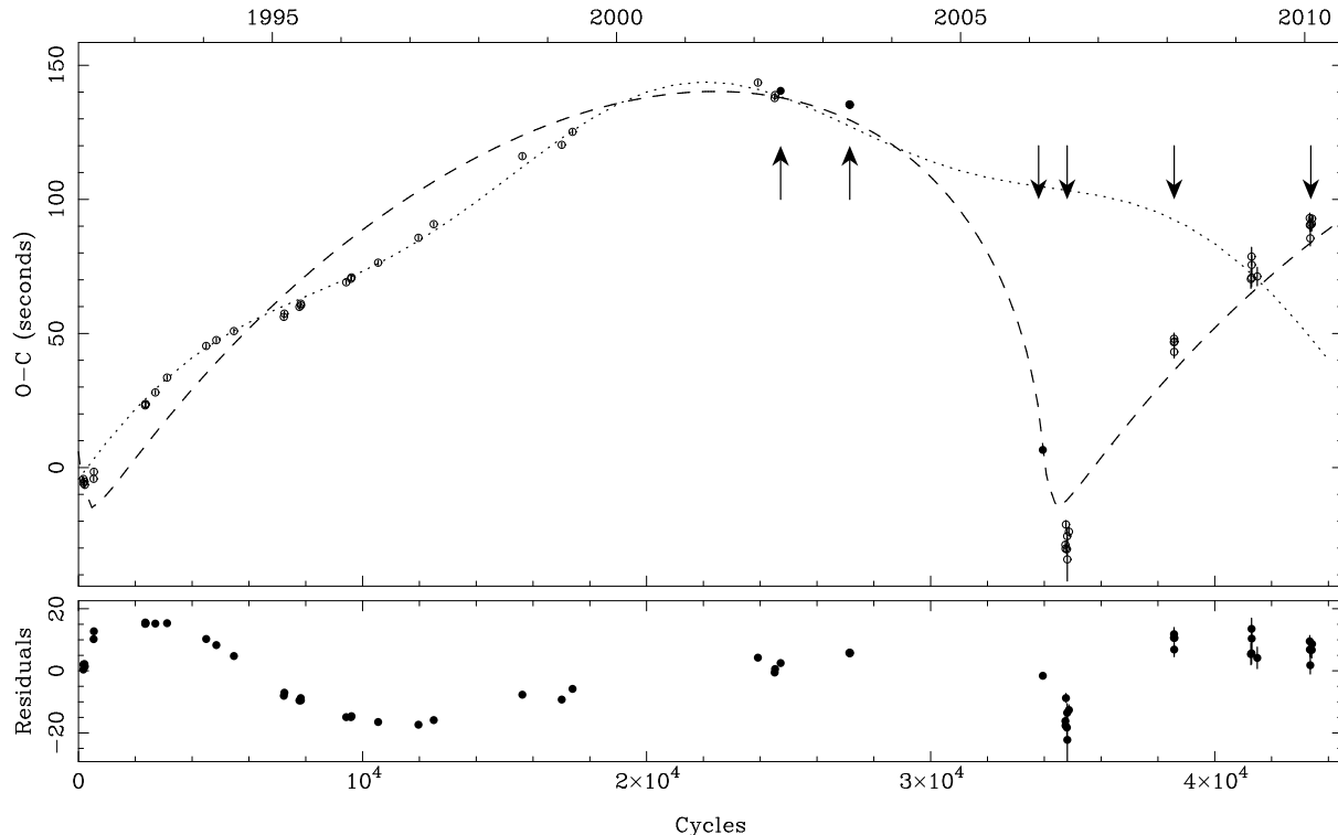
Figure 10. Top: O-C diagram for QS Vir. The ephemeris was determined by varying the ephemeris of O’Donoghue et al. (2003) in order to fit a third body in an elliptical orbit ( dashed line). We also include the sinusoidal fit from Qian et al. (2010) ( dotted line). Our additional eclipse times, indicated by the arrows, clearly disagree with the sinusoidal fit. Bottom: residuals of the fit to the third body in an elliptical orbit. The filled circles are the ULTRACAM eclipse points.
