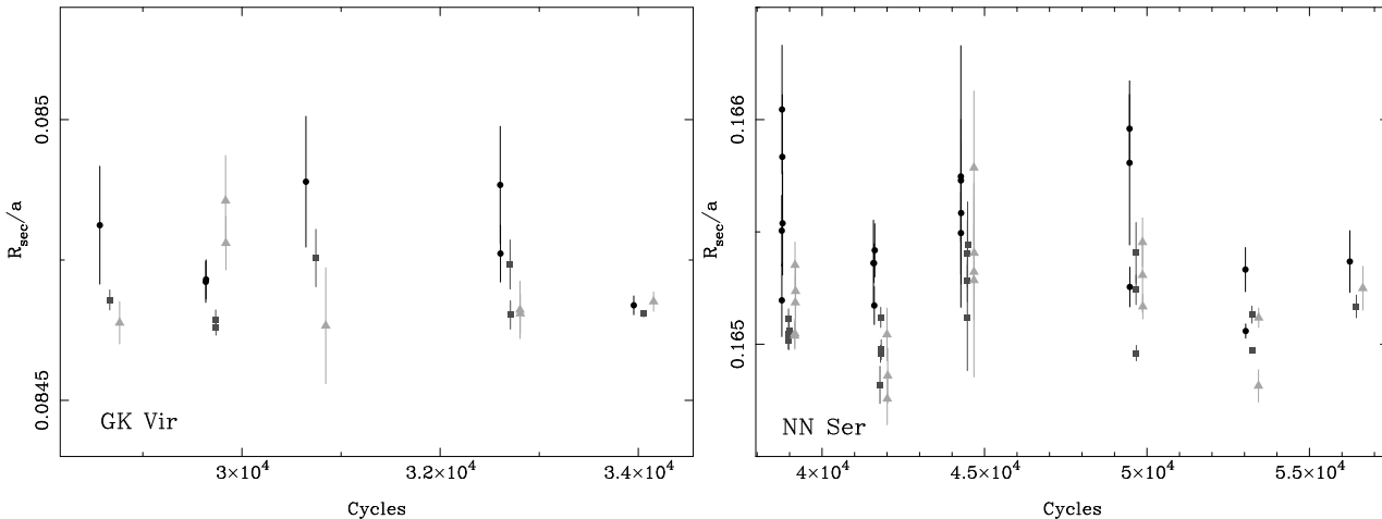
Figure 13. Measured secondary star scaled radii for GK Vir ( left ) and NN Ser ( right ). The black circles are the u' band measurements and have been offset by -100 cycles for GK Vir and -200 cycles for NN Ser. The dark grey squares are the g' band measurements and the light grey triangles are the red band ( r' or i' ) measurements and have been offset by +100 cycles for GK Vir and +200 cycles for NN Ser.
