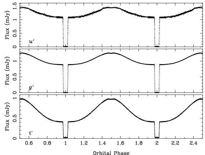
Figure 3. Full orbit light curves of NN Ser in (top to bottom) u' band, g' band and i' band. NN Ser shows a large reflection effect. Smaller bins were used around both the primary and secondary eclipses.
