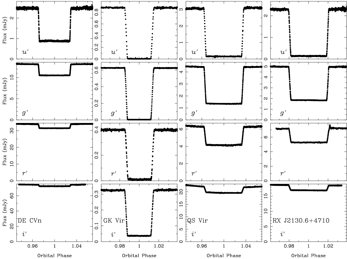
Figure 1. Flux calibrated primary eclipses of (left to right) DE CVn, GK Vir, QS Vir and RX J2130.6 + 4710 in (top to bottom) u' band, g' band, r' band and i' band. Light curves were made by phase binning all available eclipses then combining them. Any flares were removed before the light curves were combined with the exception of RX J2130.6 + 4710 in the r' band where there was only one eclipse which featured a flare.
