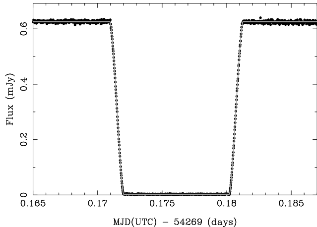
Figure 6. Light curve and model fit to the primary eclipse of GK Vir observed on 2007 June 18.
