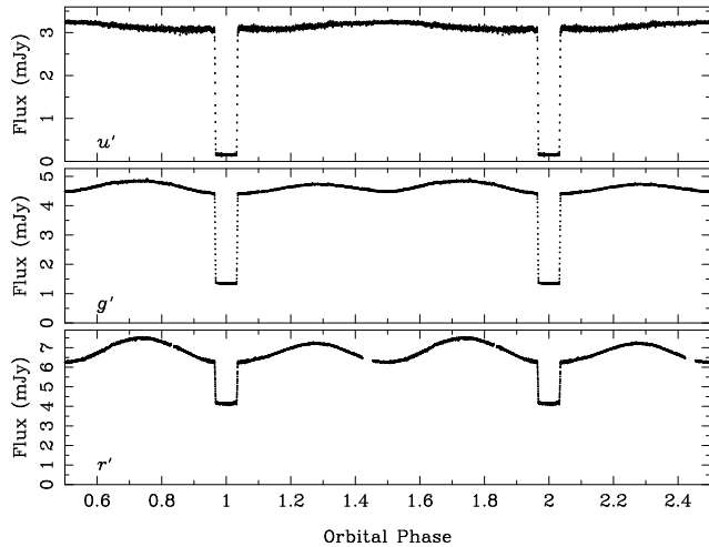
Figure 4. Full orbit light curves of QS Vir in ( top to bottom ) u' band, g' band and r' band. A small reflection effect is visible in the u' band light curve whilst ellipsoidal modulation is clearly seen in the g' and r' band light curves.
